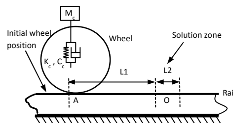
Fig. 5 The vehicle–track model in longitudinal –vertical direction
