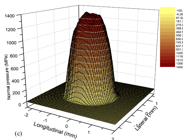
Fig. 7 Distributions of contact pressure for (a) Case-1, actual wheel-rail, (b) Case-2, 1/5 scaled test rig, (c) Case-3, 1/7 scaled test rig
