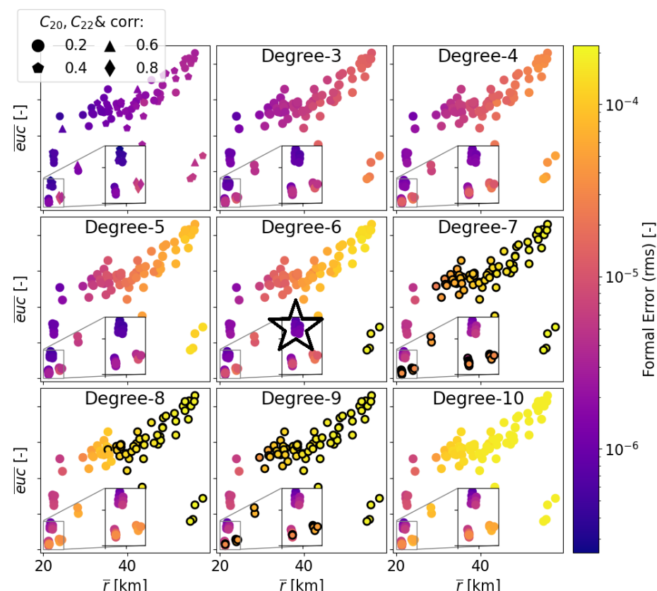
Figure 7. Gravity field recovery for the combined experiment. RS tracking is 12 h/day, CG sensitivity is \sigma_\gamma = 37.5 \text{ mE} \sqrt{\text{Hz}} with measurements every 11 s. Shapes reflect the correlation between C_{20} and C_{22} . In contrast to Figure 5, here all the formal errors stay below the a-priori standard deviations, hence the circled markers indicate that the formal errors cross the homogeneous values. The star denotes the best (family of) orbits in terms of accuracy across degrees 4 to 10.
