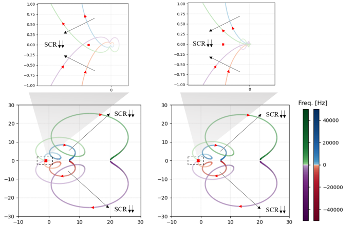
Fig. 5. Eigen-loci the \mathbf{L} of the grid-charger system with different SCR. The red-blue curves are the eigen-loci when SCR=8.4 whereas the purple-green curves are the eigen-loci when SCR=2.8 . Clearly, when the SCR is small, the grid-charger system is unstable because the -1+j0 point is encircled by the eigen-locus shown on the left-hand side.
