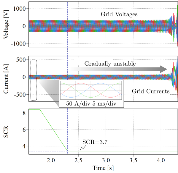
Fig. 7. Simulation shows the charging system is unstable when the SCR is just below the derived CSCR_s .
