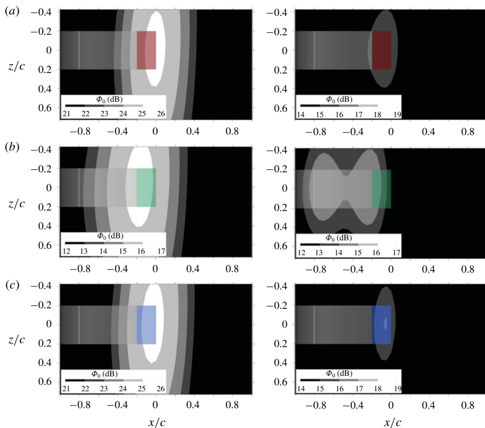
FIGURE 11. Source maps for one-third octave band, centred at 1250 Hz ( St_c = 12.5 ) (left column) and 2500 Hz ( St_c = 25 ) (right column) for the (a) solid, (b) porous and (c) blocked TE cases. The trailing-edge region ( -0.2 < x/c < 0 ) for each respective case is highlighted in different colours.
