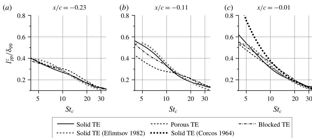
FIGURE 19. Spanwise coherence length ( l_{pp}^z ) plotted against the chord-based Strouhal number ( St_c ). For comparison, predictions of the Corcos (Corcos 1964) and Efimtsov models (Efimtsov 1982; Palumbo 2012) are included.
