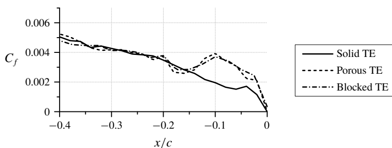
FIGURE 24. Streamwise distribution of mean wall-friction coefficient C_f for the different trailing-edge cases.
