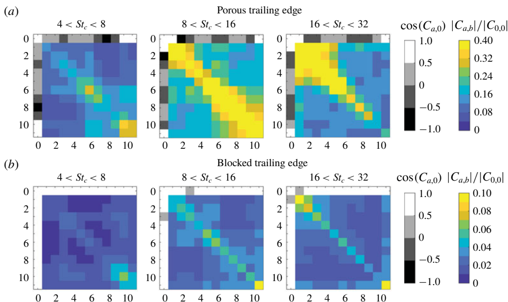
FIGURE 16. Normalized cross-spectral density (CSD) (inner coloured matrix) for the various strips and the resulting phase information (outer grey scale matrix) with respect to the overall trailing-edge region. Note that colour bars of (a) and (b) have different scales.
