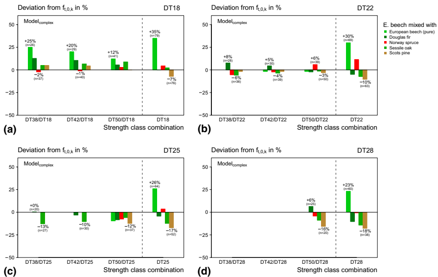
Fig. 6 Deviations of the characteristic strength value from the required characteristic strength values for DT-classes DT18 (a), DT22 (b), DT25 (c) and DT28 (d) using Model_{complex} . The bold figures next to the bars are the most positive and negative deviation among the mixture types for each combination, numbers in brackets are the number of boards. Bars are only illustrated if more than 20 boards were available. (Color online)
