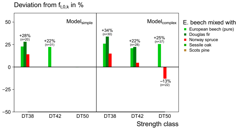
Fig. 4 Deviations of the characteristic strength value from the required characteristic strength values for DT38, DT42 and DT50 using \text{Model}_{\text{simple}} (left) and \text{Model}_{\text{complex}} (right). The bold figures next to the bars are the most positive and negative deviation among the mixture types for each combination, numbers in brackets are the number of boards. Bars are only illustrated if more than 20 boards were available. (Color online)
