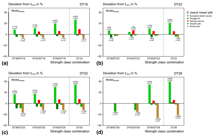
Fig. 5 Deviations of the characteristic strength value from the required characteristic strength values for DT-classes DT18 (a), DT22 (b), DT25 (c) and DT28 (d) using \text{Model}_{\text{simple}} . The bold figures next to the bars are the most positive and negative deviation among the mixture types for each combination, numbers in brackets are the number of boards. Bars are only illustrated if more than 20 boards were available. (Color online)
