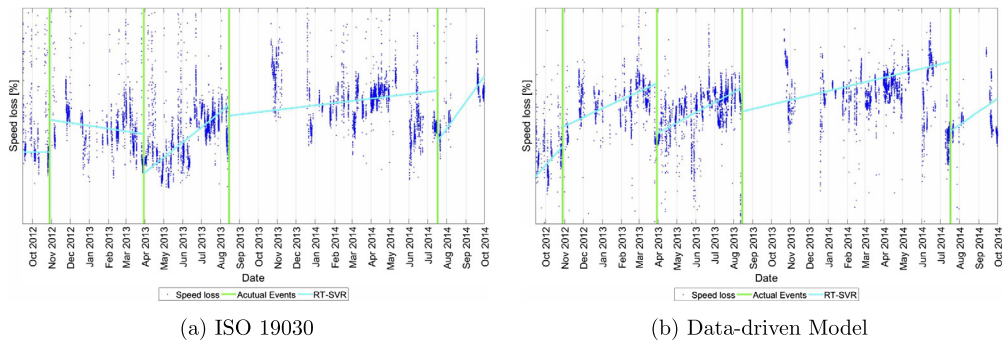
Figure 7.7 Case Study 2 – Robust Regression Analysis on the Speed Loss Percentages between two consecutive Hull and Propeller Cleaning Events for V1.
