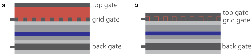
Figure 3.6: Two distinct device designs for imposing a periodic potential. Either the grid and top gate are separated by a thick dielectric (a), rendering their capacitance small enough to be neglected, or they are separated only by the oxidation of the first layer (b), in which case their capacitance is much larger than the device capacitance and the two gates can be seen as one from the perspective of the A/C measurement signal.
