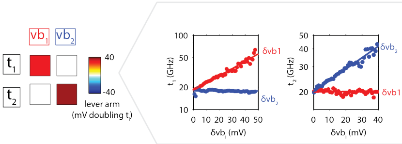
Figure 4.10: Controlling one tunnel coupling at a time. Compensating for the cross-talk measured in Fig 4.4, we can define barrier gates vb_i that influence only one tunnel coupling at a time. (add mV to x-label!)
