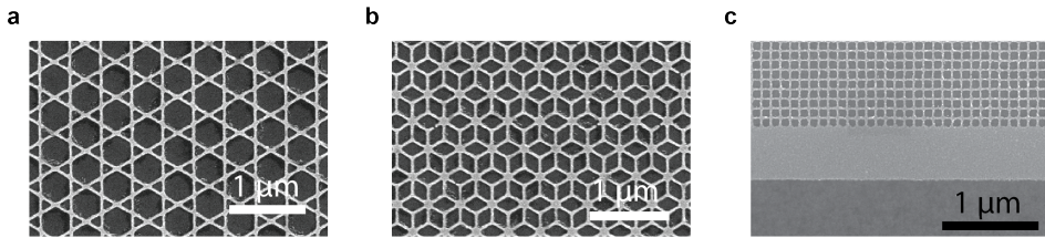
Figure A.2: Nano-fabricated grids. Electron micrographs of metallic ( 20\text{ nm} of Al, light) grid-shaped gates fabricated on GaAs (darker background). Besides square grids, kagome (a) and dice-shaped lattices can also be fabricated (b). Homogeneity at the edges is provided for by overdosing a thin frame at the edge, as shown in c.
