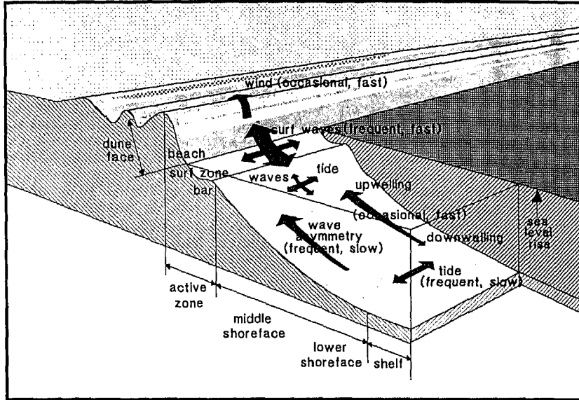
Figure 3 Overview of sediment transport processes in a coastal cell along the closed coast
