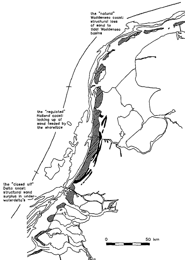
Figure 1 Three subsystems of the coast of the Netherlands
