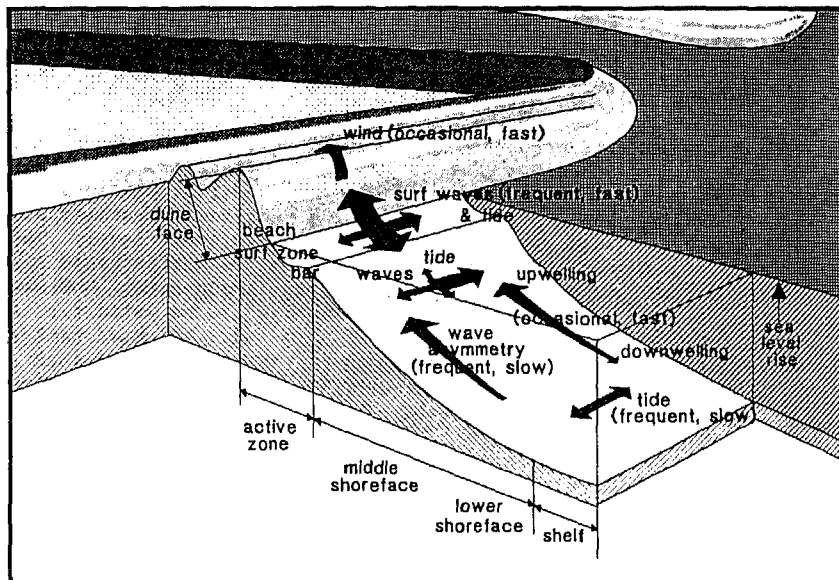
Figure 4 Overview of sediment transport processes in a coastal cell along a coast interrupted by a coastal inlet
