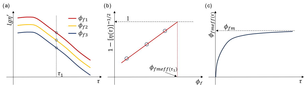
Figure 2. (a) Flow curves of FR-CPB varying in fiber dosages ( \phi_{f1} , \phi_{f2} , \phi_{f3} ) under stress ramp-up tests [29]; (b) \phi_{fmeff}(\tau_1) corresponding to the fiber configuration under \tau_1 [29]; (c) determination of \phi_{fm} [29].
