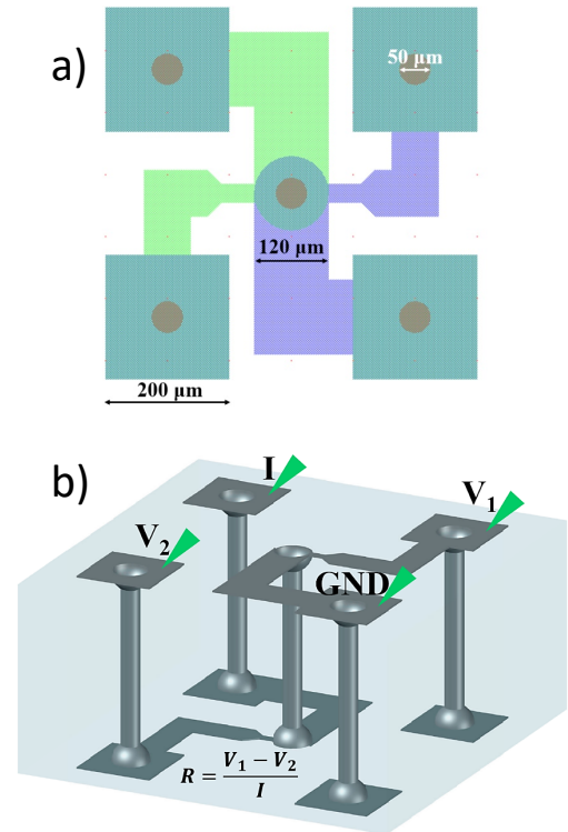
Figure 6: Sketches of the cross-bridge Kelvin resistor test structure used for the electrical characterization of the Al/TiN TSVs. a) Layout of the test structure and b) 3D sketch of the structure and electric measurement setup.
