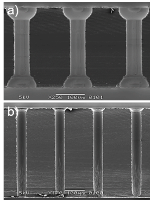
Figure 3: Scanning electron microscope (SEM) cross-sectional view of 50 \mu\text{m} wide TSVs on a a) 300 \mu\text{m} -thick Si wafer b) 500 \mu\text{m} -thick Si wafer.
