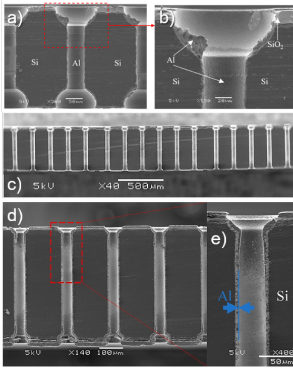
Figure 4: SEM cross-sectional view of the realized TSVs: a) a 300 \mu\text{m} -deep, 50 \mu\text{m} -wide via after Al/TiN sputtering, b) close-up of a funnel evidencing the composition of the material layers; c) an array of 500- \mu\text{m} deep, 50 \mu\text{m} -wide TSVs after Al sputtering, and d) close-up of Al/TiN-coated TSVs evidencing the composition of the material layers (e).
