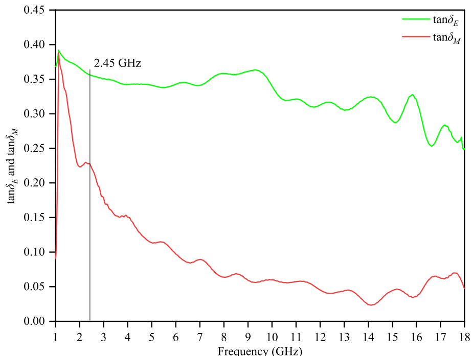
Fig. 12. Test results of the dielectric loss tangent and magnetic loss tangent of PCB.
