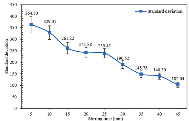
Fig. 18. Effect of stirring time on uniformity of PCB.
