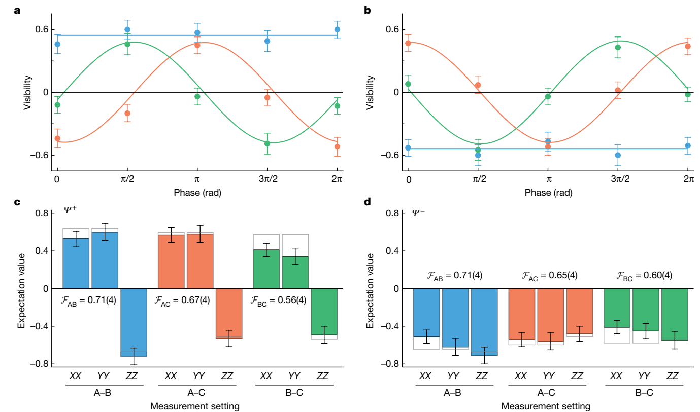
Fig. 4 | Concurrent entanglement generation in the network. a,b , Measured correlation \langle XX \rangle of |\psi^+\rangle ( a ) and |\psi^-\rangle ( b ) on three links when changing the phase \theta at Charlie. Blue, orange and green data points refer to the results of the Alice–Bob, Alice–Charlie and Bob–Charlie links, respectively. The curves show the
