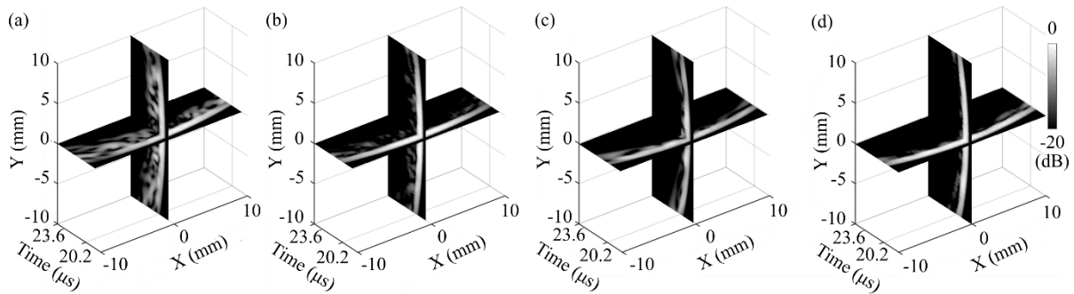
Fig. 3. Field II simulations of the one-way field obtained for 2\alpha = 30^\circ divergent angle at 3 cm away from the transducer, displayed at a dynamic range of 20 dB normalized to their maximum amplitudes. (a) Transmitting with all elements. (b) Transmitting 5 partially overlapping beams with all elements. Four beams all with 5^\circ steering angle were transmitted into different directions centered around a non-steered beam. The transmitted waves were simulated separately, corrected for time-of-flight differences and averaged, then mapped onto the wave-front locations of the non-steered transmit. (c) Transmitting one un-steered beam with the center 120 elements. (d) Transmitting with the center 120 elements and with the same steering configuration as in (b).
