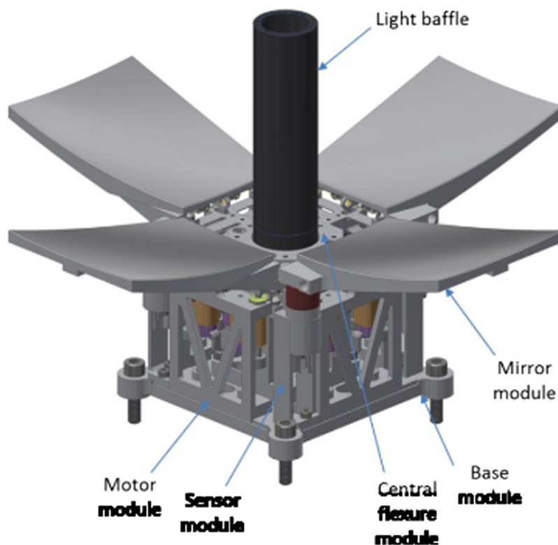
Fig. 11 Schematic representation of the adjustment mechanism of the deployable telescope proposed by Schwartz et al. 95 showing an additional internal baffle.
