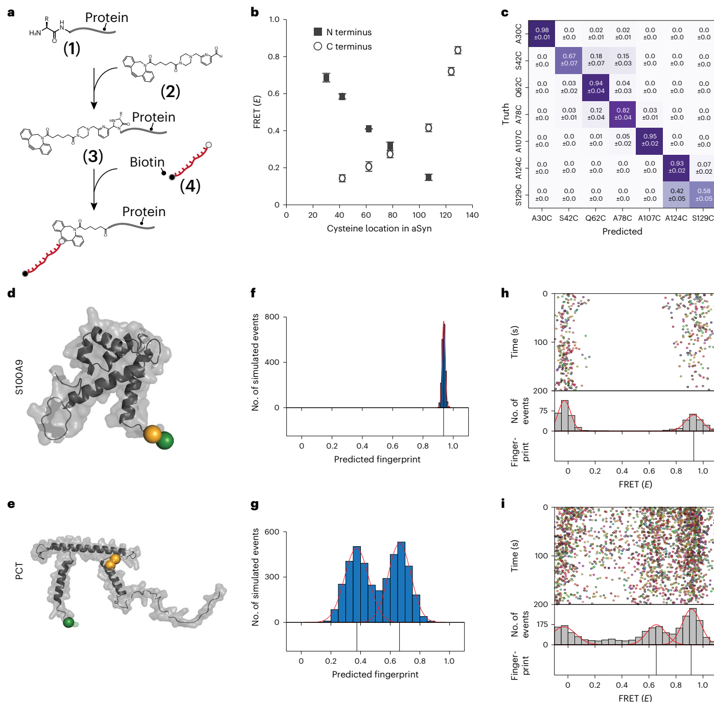
Fig. 4 | Single-molecule protein fingerprinting using N-terminal labelling.
