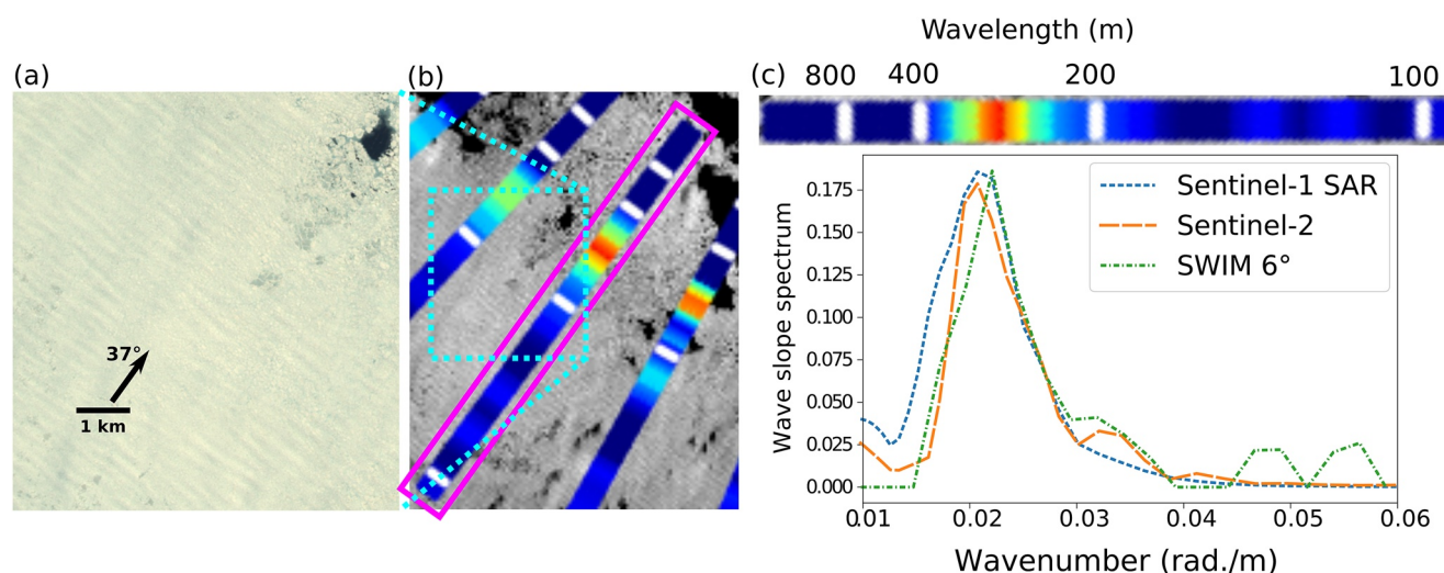
Figure 10. (a) and (b) Wave patterns around 76.7°N, 30°E on 12 March 2021, and CFOSAT-SWIM spectrum in azimuth 37° using the 6° incidence beam, compared to the spectra of Sentinel-1 and Sentinel-2 images in the same region. In (b) SWIM modulation spectra from the 6° incidence beam are overlaid as colored strips. The white marks in the colored strip correspond to wavelengths 800, 400, 200, and 100 m. (c) SWIM spectrum for the azimuth 37° clockwise from North in strip form as a the usual power spectral density as a function of wavenumber, compared with spectra in the same direction from Sentinel-1 and Sentinel-2 imagery. ICESat-2 data was averaged from the three strong beams over the latitude range 77.75°–77.9° using Fourier transforms over 0.05° in latitude. The wavenumber was multiplied by the proper projection from the satellite track to the 37° azimuth, common to the other data sets.
