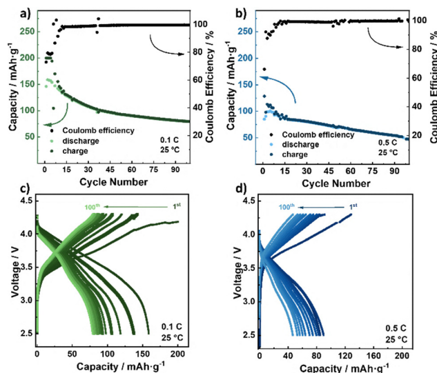
Fig. 5 Full cell performance of \text{LPSCl}_{1.5}@\text{GCD-PCL}@\text{PA} in the potential range from 2.6 V to 4.3 V at 25 ^{\circ}\text{C} , a pressure of 50 MPa and a current density of 0.18 \text{mA cm}^{-2} (0.1C) and 0.90 \text{mA cm}^{-2} (0.5C). A 70 wt% : 30 wt% mixture of \text{NCM}_{83} and \text{LPSCl}_{1.5} was used as the cathode composite. The anode composite was a mixture of Si/C and \text{LPSCl}_{1.5} in a weight ratio of 55 : 45. (a) and (b) Capacity retention and Coulomb efficiency over 100 cycles at 0.1C and 0.5C. (c) and (d) Charge and discharge curves for every 10th cycle (1st, 10th, ..., 100th) at 0.1 and 0.5C.
