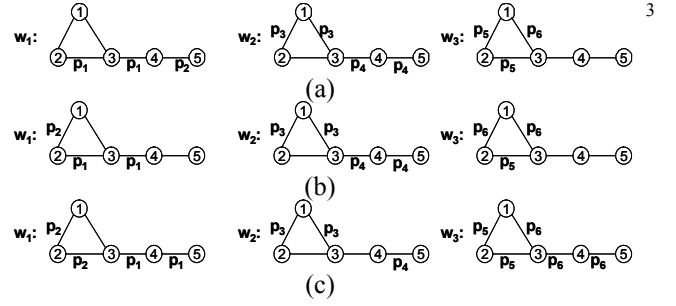
Fig. 3. Different scenarios of wavelength rerouting: (a) moving to vacant, (b) sequential rerouting, and (c) swapping.
