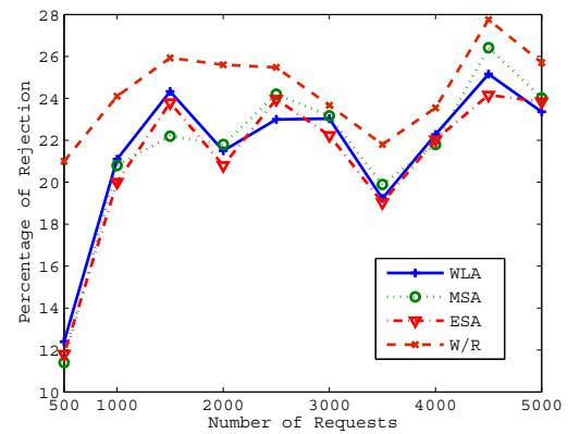
Fig. 8. Rejection rate of MSA , ESA , WLA and without rerouting for different number of requests for the random network. ( N = 50 , \alpha = 0.2 , W = 10 , r = 120 )
