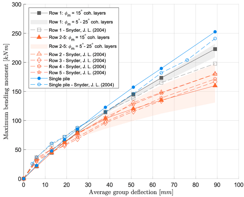
Fig. 16. Comparison of maximum bending moment vs. average group deflection. Pile group is computed with \varphi_m = \varphi for granular layers and \varphi_m = 15 deg. for cohesive layers with a bandwidth of \pm 10 deg.
