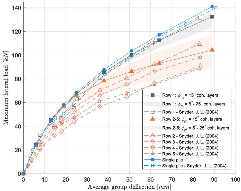
Fig. 15. Comparison of average pile row load vs. applied group deflection. Pile group is computed with \varphi_m = \varphi for granular layers and \varphi_m = 15 deg. for cohesive layers with a bandwidth of \pm 10 deg.
