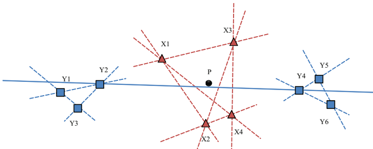
Figure 4.1: Interpolation inaccuracy
