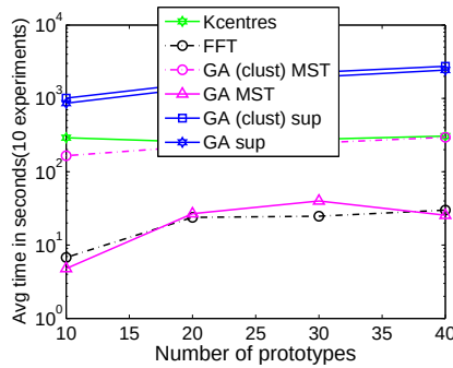
(e) SVHN
