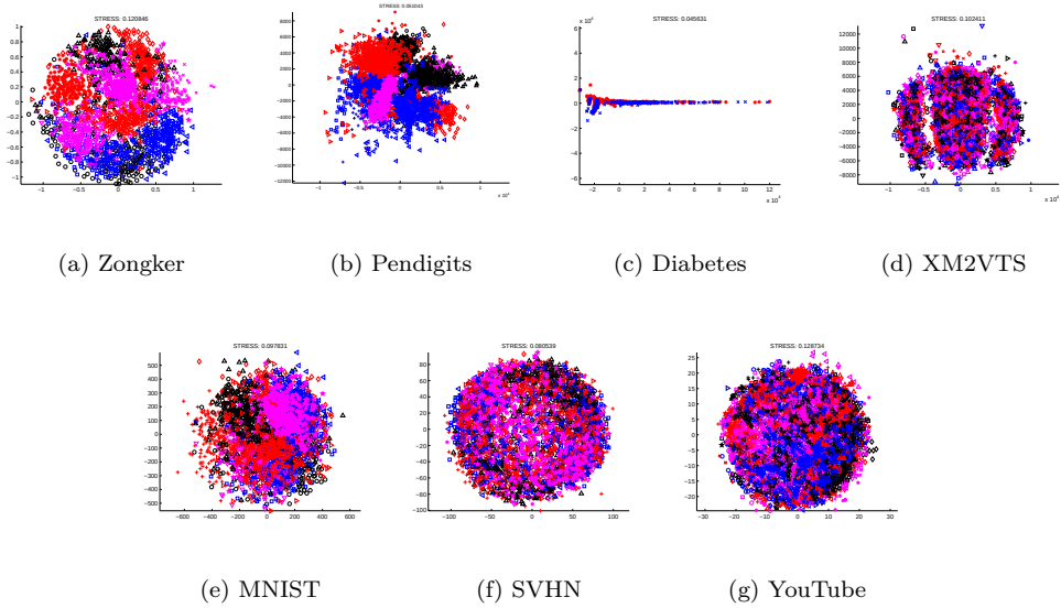
Figure 3.10: MDS mappings
