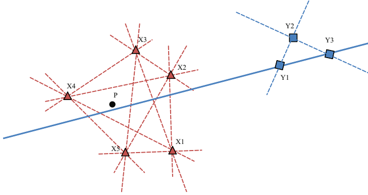
Figure 4.2: Extrapolation inaccuracy
