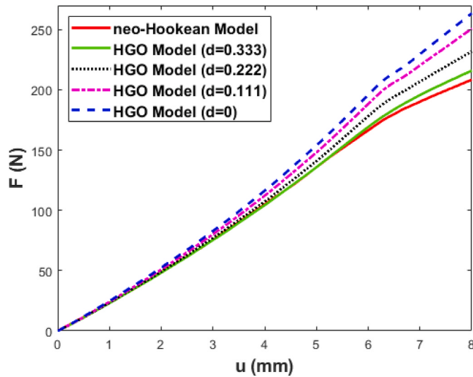
Fig. 9. Influence of fibre dispersion in TA on the overall response of penile tissue in compression testing ( \alpha = 90 ).
