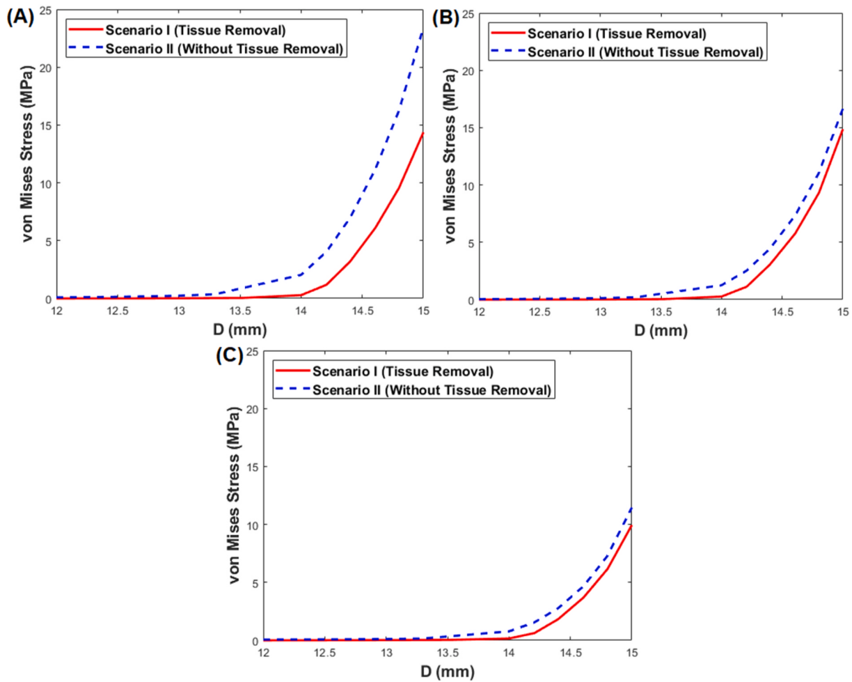
Fig. 11. Comparison of von-Mises stresses between two IPP implantation scenarios when neo-Hookean hyperelastic model is used for all tissue layers, (A) point 1 (Inn_CC), (B) point 2 (Out_CC), and (C) point 3 (Mid_TA).
