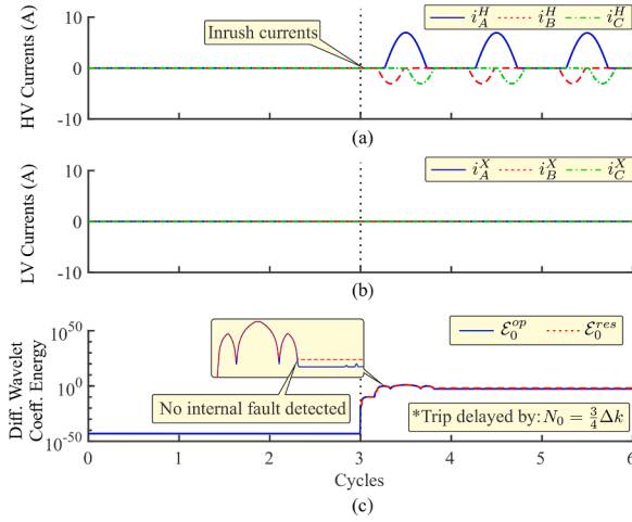
Fig. 7. Transformer energization: (a) i_A^H , i_B^H , i_C^H ; (b) i_A^L , i_B^L , i_C^L ; (c) Zero-mode differential energies \mathcal{E}_0^{op} and \mathcal{E}_0^{res} .
