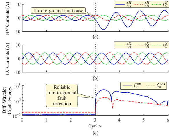
Fig. 3. Turn-to-ground fault: (a) i_A^H , i_B^H , i_C^H ; (b) i_A^X , i_B^X , i_C^X ; (c) Zero-mode differential energies \mathcal{E}_0^{op} and \mathcal{E}_0^{res} .
