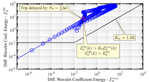
Fig. 6. Zero-mode energy operating points during one cycle of the transformer energization with turn-to-ground fault.
