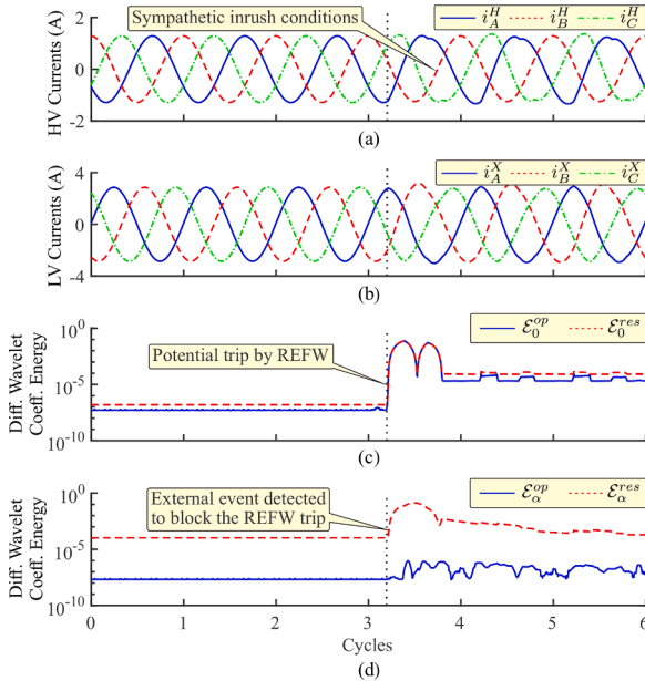
Fig. 9. Sympathetic inrush condition: (a) i_A^H , i_B^H , i_C^H ; (b) i_A^L , i_B^L , i_C^L ; (c) Zero-mode differential energy components \mathcal{E}_0^{op} and \mathcal{E}_0^{res} . (d) Alpha-mode differential energy components \mathcal{E}_\alpha^{op} and \mathcal{E}_\alpha^{res} .
