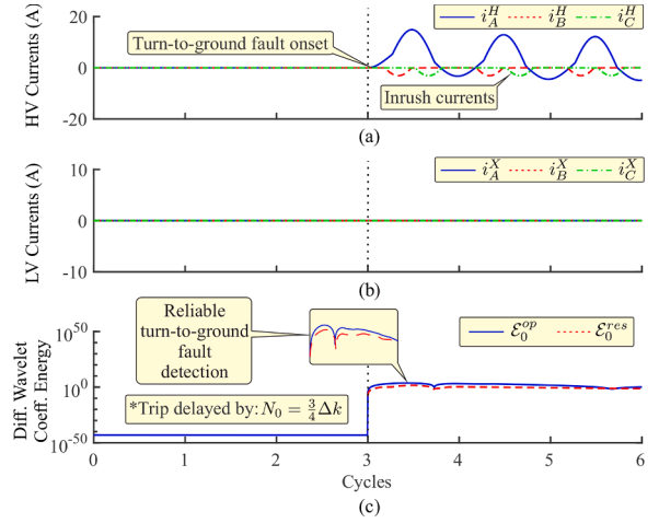
Fig. 5. Transformer energization with turn-to-ground fault: (a) i_A^H , i_B^H , i_C^H ; (b) i_A^X , i_B^X , i_C^X ; (c) Zero-mode differential energies \mathcal{E}_0^{op} and \mathcal{E}_0^{res} .
