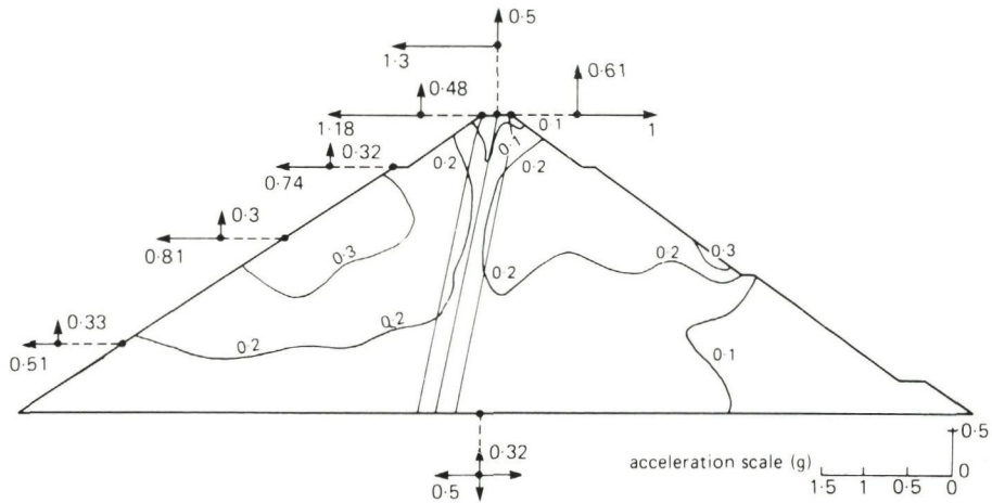
Fig. 5.10 Computed maximum accelerations and cyclic shear strains caused by combined horizontal and vertical base motions
