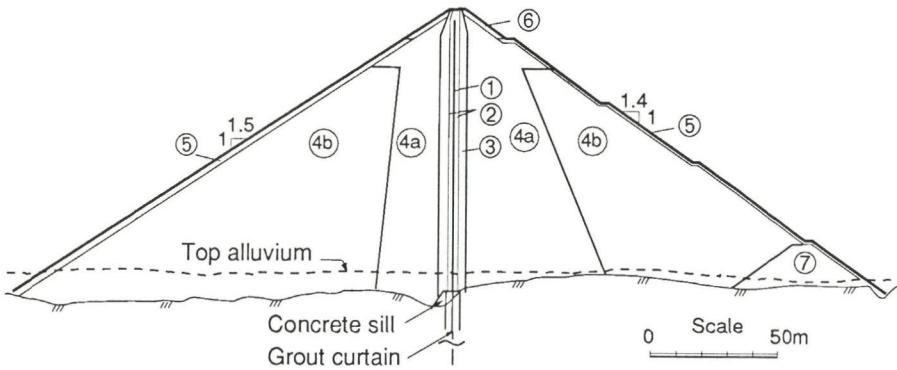
Fig. 3.1 Site and cross section of Storglomvatn Dam
