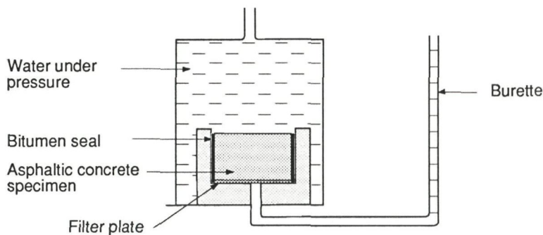
Fig. 6.9 Permeability testing
