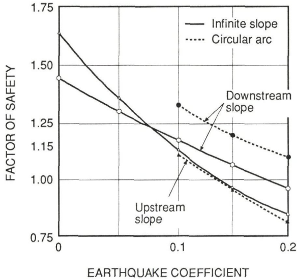
Fig. 5.8 Results of pseudo-static stability analysis
