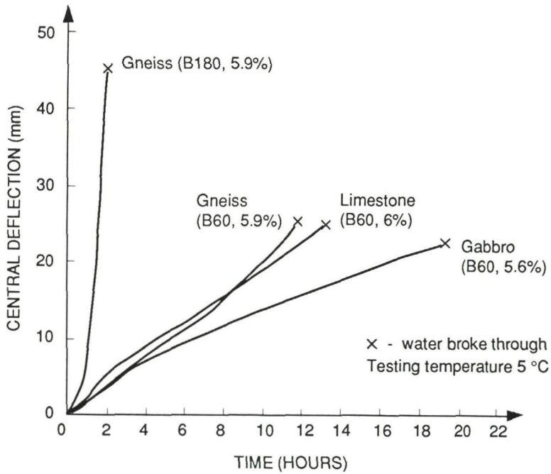
Fig. 6.11 Results from plate permeameter tests
