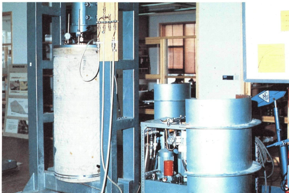
Fig. 5.4 NGI's large vacuum triaxial test
