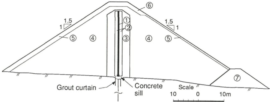
Fig. 3.8 Langavatn Dam
