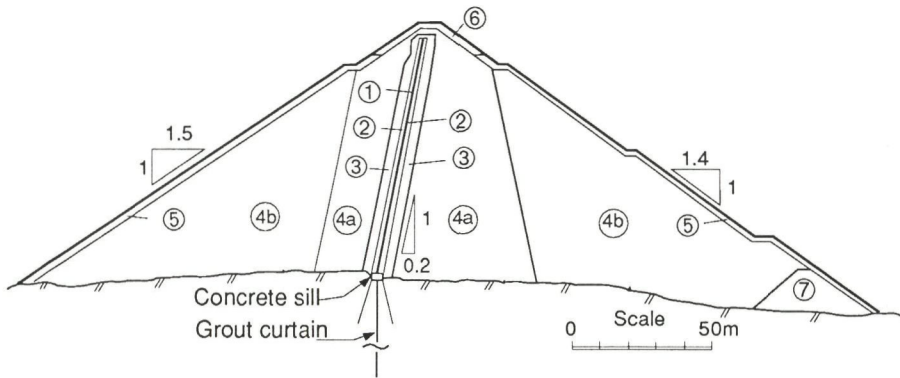
Fig. 3.2 Storvatn Dam
