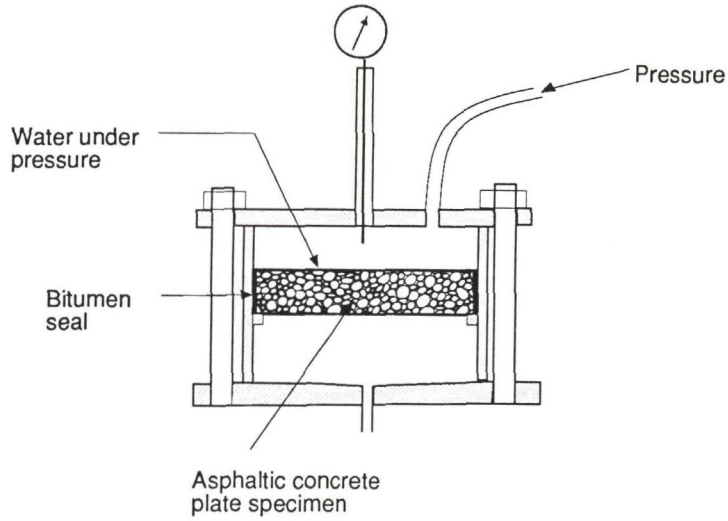
Fig. 6.10 Sketch of the NGI plate permeameter
