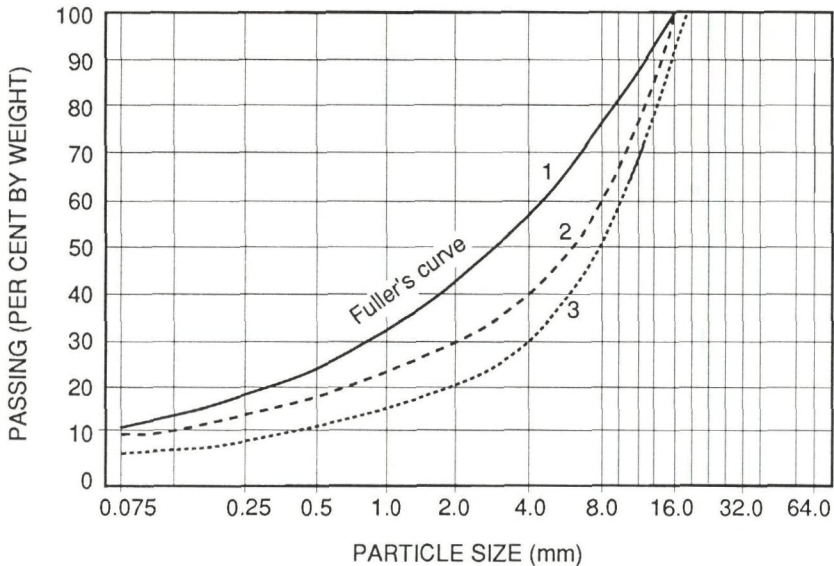
Fig. 6.3 Fuller's gradation curve for asphaltic concrete aggregates
