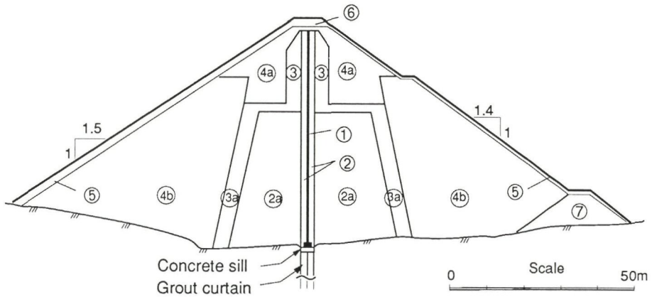
Fig. 3.3 Berdalsvatn Dam
