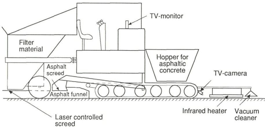
Fig. 4.3 Working principle for core paver
