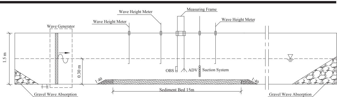
Figure 1. Schematic design of the wind-wave-current flume and the layout of measured instruments.
