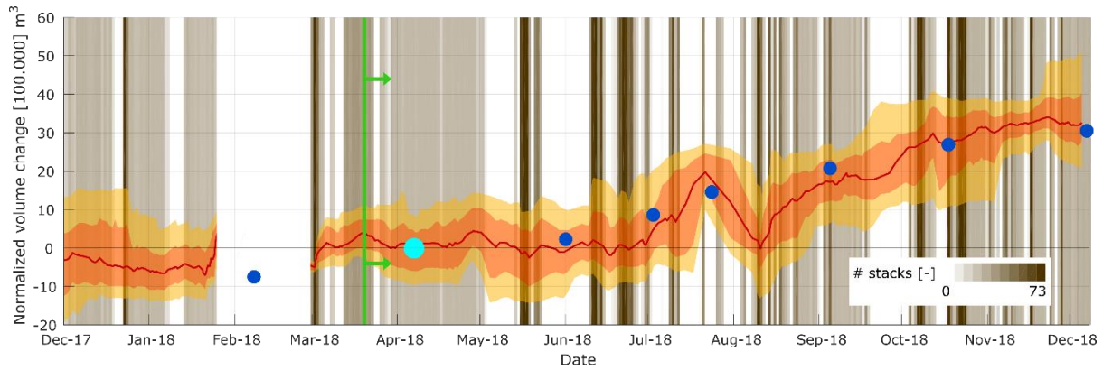
Figure 8. The time-evolution of the sediment volume changes in the nourishment area (Figure 6, green polygon) for the period Dec 2017 – Dec 2018 according to radar (red line) and multibeam surveys (blue dots). Volume changes are normalized to the 2 nd multibeam survey (cyan dot). Per day, the number of available XMFIt results that covered the nourishment area - and could hence be used for volume calculations - is indicated by a vertical grey band (see colorbar). The monthly median radar estimate (red line) is presented with corresponding 25 – 75 percentile range (shaded red) and 10 th – 90 th percentile range (shaded yellow). The start of nourishment execution, 20 Mar. 2018, is indicated by the vertical green line.
