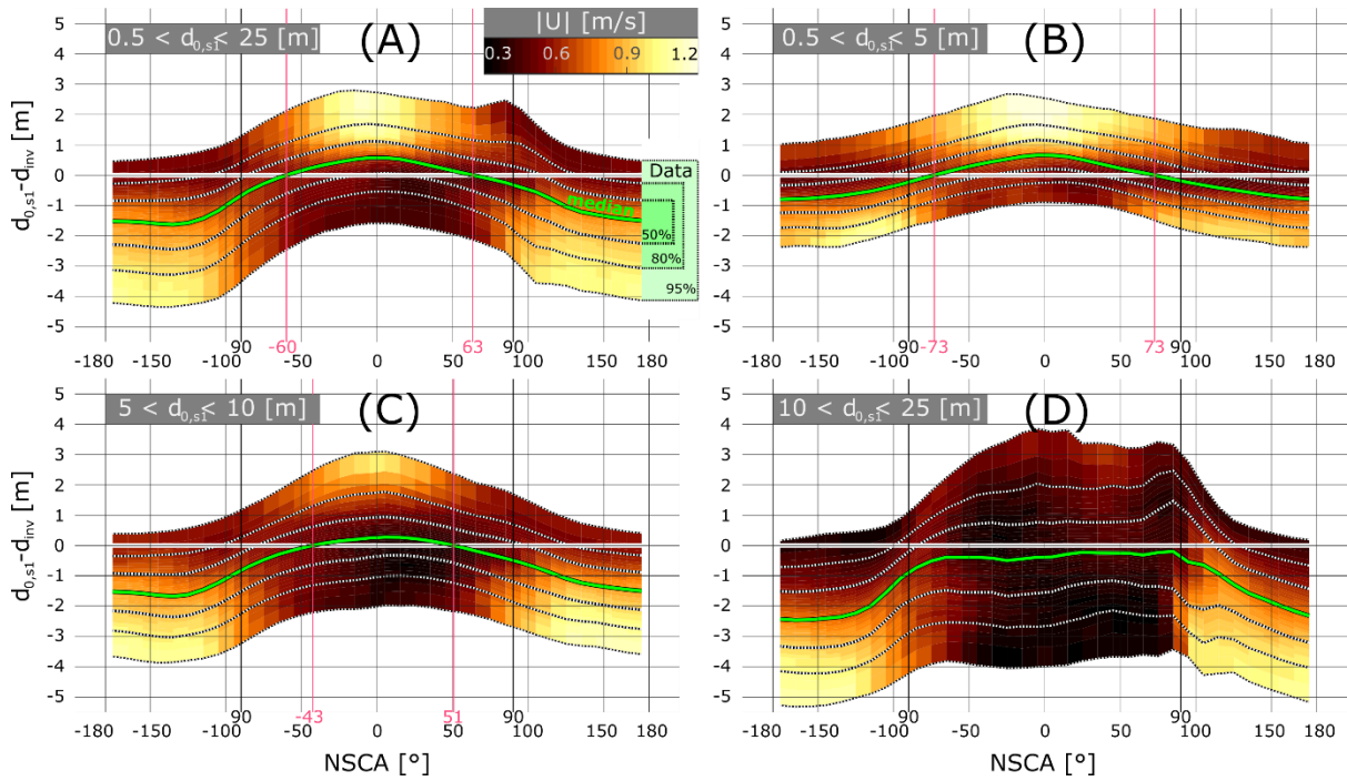
Figure 10. Observed depth bias (vertical axis) as a function of the near-surface current angle (NSCA) with respect to mean wave direction (horizontal axis). At NSCA = \pm 0^\circ , near-surface currents point in direction of wave propagation, whereas for NSCA = \pm 180^\circ they oppose each other. The depth bias is used as proxy for the depth error. Corresponding near-surface current magnitudes ( |U| ) are shown in bronze colors (colorbar). Panels present data within different ranges of depth: a) 0.5 < d_{0,s1} < 25.0 m (all data); b) 0.5 < d_{0,s1} < 5.0 m; c) 5.0 < d_{0,s1} < 10.0 m;
