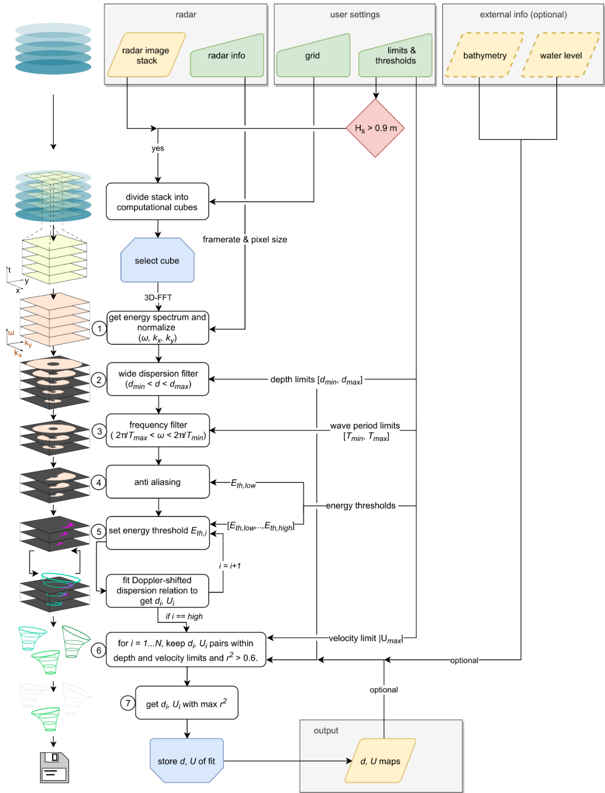
Figure 1. XMFit workflow for depth and near-surface current inversion from an image sequence. Consecutive processing steps in the flowchart are visualized along their left. The flowchart includes: data (brown), user input (green), decision (red), process loop start (blue;
