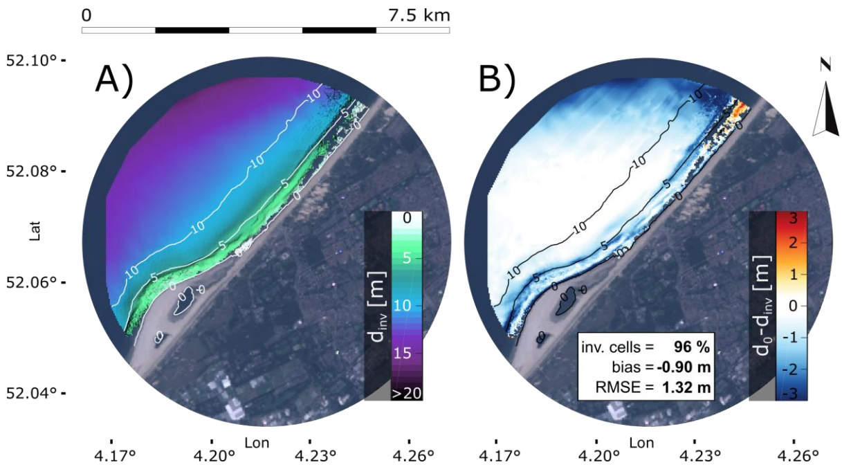
Figure 4. Radar-derived results for the Sand Engine. (a) Inverted depths d_{inv} (m) (colorbar). (b) Comparison of d_{inv} against in-situ measured depths d_0 (m), where red/blue colors indicate under-/overestimation of depth respectively. In both panels, contour lines of measured depths are superimposed for reference. Results represent the median over 184 image sequences spanning 18 h in total. Values are included for the percentage of grid cells returning a result (inv. cells), the overall bias (bias) and the root mean squared error (RMSE).
