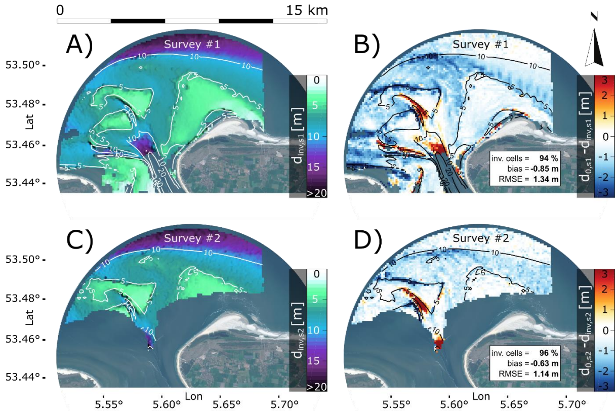
Figure 5. XMFit results from the operational Ameland system as compared to a survey from 31- May to 5- June 2018 (Survey #1) and a survey from 12-14 October 2018 (Survey #2). Panels (a,c): average depth estimates over two days encompassing each survey, as indicated by (a) d_{inv,S1} for Survey #1 and (c) d_{inv,S2} for Survey #2. Single beam observations are outlined by white depth contours. Panels (b,d): difference of inverted depths d_{inv} with the corresponding single beam measurements d_0 (now accentuated by black contours instead of white contours) as indicated by (b) d_{0,S1} - d_{inv,S1} for Survey #1 and (d) d_{0,S2} - d_{inv,S2} for Survey #2. Similar to the Sand Engine a mostly negative bias (depth overestimation; blue) is observed, being a little higher for Survey #1 (bias = -0.85 m) than Survey #2 (bias = -0.63 m).
