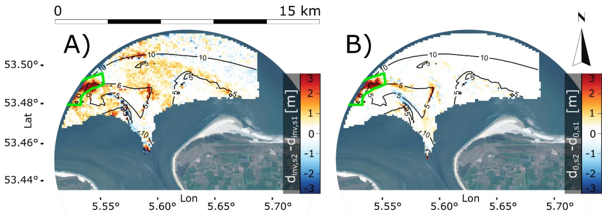
Figure 6. Difference between June (Survey #1) and October (Survey #2) as derived for radar and single beam measurements. (a) radar: inverted depths d_{inv,S1} of Survey #1 are subtracted from d_{inv,S2} of Survey #2. (b) single beam: accordingly, measurements d_{0,S1} of Survey #1 are subtracted from d_{0,S2} of Survey #2. The pilot nourishment fronting the ebb shield is clearly visible in both cases and its position is in line with expectation (green polygon). Note that the surveys do not cover the entire radar domain. For visual clarity, differences between radar results (a) are truncated to the same area as the surveys (b).
