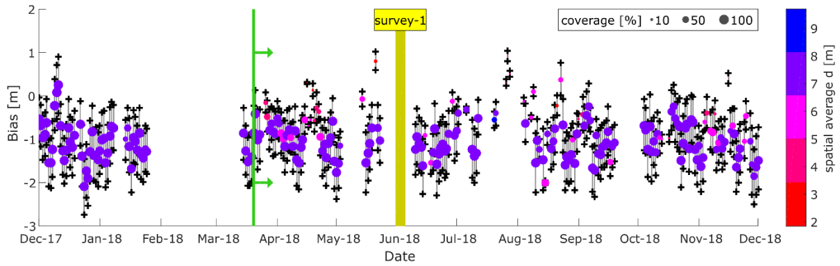
Figure 7. Mean spatial bias over the full radar domain of XMFit estimates with ground truth data surveyed between 31 May to 5 June 2018 (Survey #1, yellow). The start of nourishment works is indicated by a vertical green line. Representative bed elevations are obtained by subtracting local water level measurements from the XMFit depth estimates. Dots represent the daily median result and whiskers the corresponding 25 th and 75 th percentiles. Colors indicate the average depth over the parts of the radar image that contain results and show that the bias appears lower for moments when only small (small marker size), shallow (magenta, red) areas could be inverted. When coverage is high (large marker size) the bias also accounts for sensitive deeper parts (purple, blue). Note that the lack of data during February is due to a temporary system shutdown.
