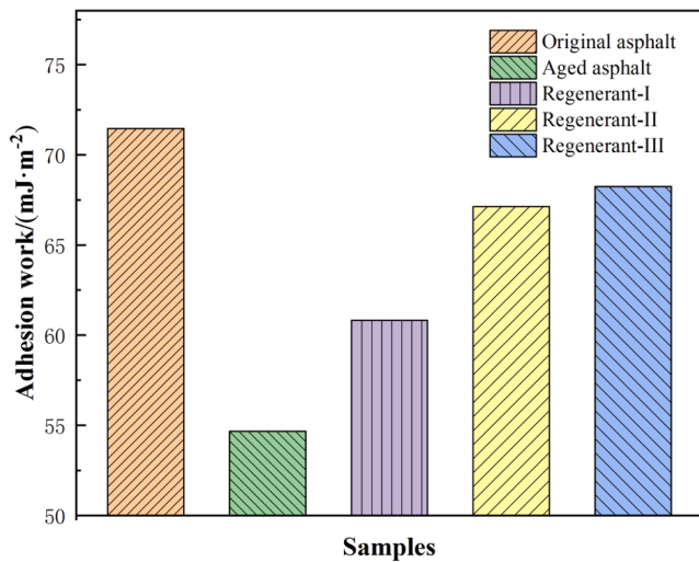
Fig. 10. Adhesion work of all modified asphalt samples.
