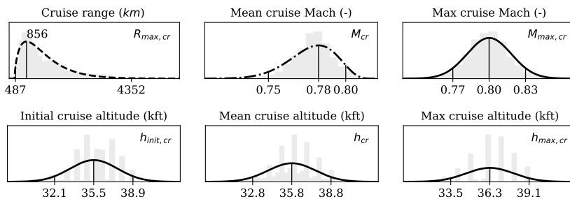
Figure 5.12: Cruise parameters
