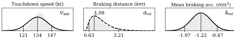
Figure 5.15: Landing parameters
