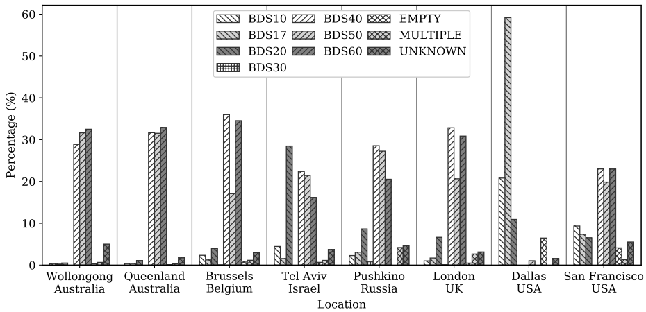
Figure 2.9: Statistics of BDS codes in Comm-B replies at different geographic regions
