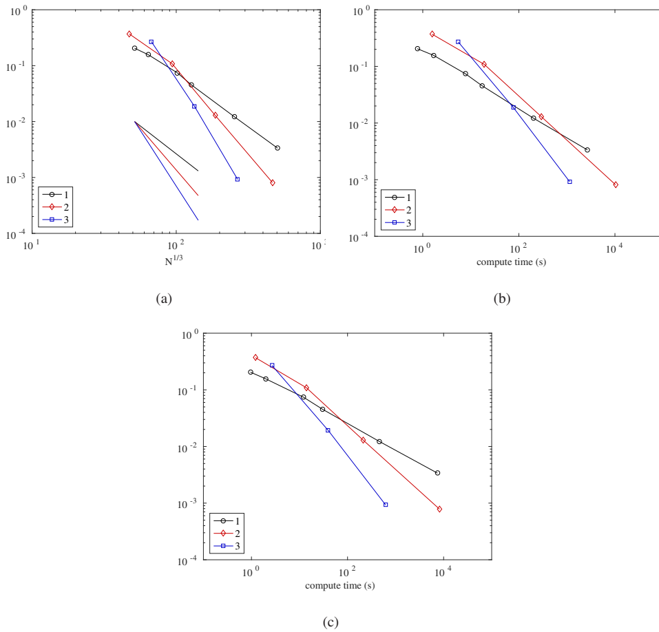
Figure 2. Maximum error in the vertical displacement, scaled by the maximum amplitude, for elements of degree 1, 2 or 3, as a function of (a) N^{1/3} , where N is the number of degrees of scalar degrees of freedom, (b) compute time with global assembly, and (c) with local assembly. The extra set of 3 short lines in (a) depicts the theoretical asymptotic error behaviour.
