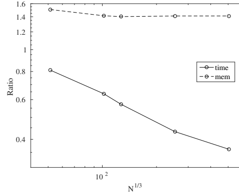
Figure 1. Ratios for compute time (drawn line) and storage (dashed) with linear elements as a function of N^{1/3} , where N is the number of nodes on the mesh. The results for the globally assembled case were divided by those for locally assembled stiffness matrices. The latter requires less storage, but is slower. The obtained reduction in storage does not seem to justify the larger compute times with linear elements.
