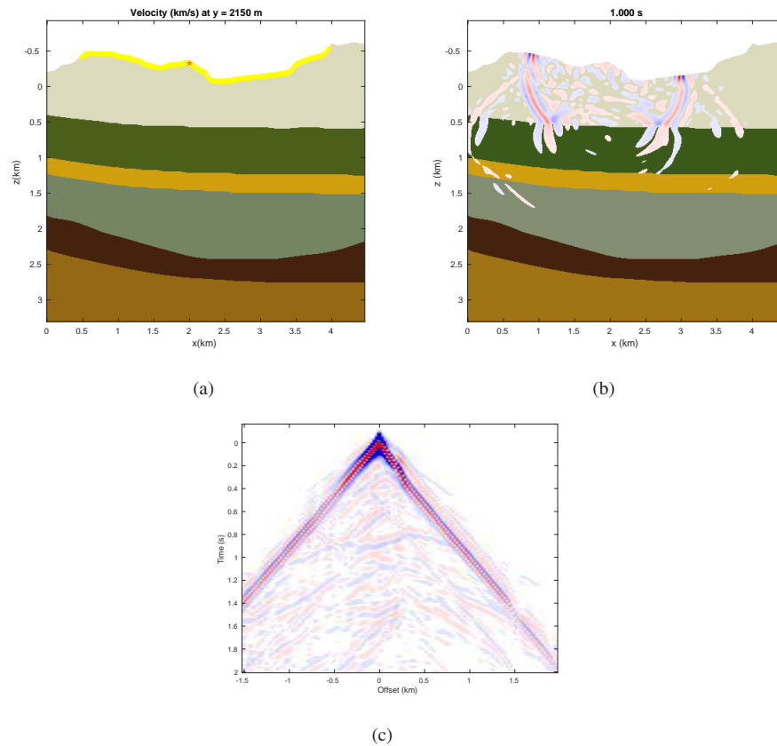
Figure 4. (a) P-wave velocities in km/s. The red star denotes the source positions and the yellow inverted triangles the receivers. (b) Vertical-displacement wavefield after 1 second. (c) Seismogram with vertical displacement.
