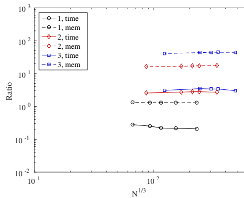
Figure 5. Ratios between compute time (drawn lines) and required storage (dashed lines) for global assembly and local assembly on the fly with elements of degree 1, 2 or 3. As in Figure 3, global assembly is faster for degree 1 at 30 to 40% more storage, whereas for degrees 2 and 3, local assembly is faster and requires substantially less storage.
