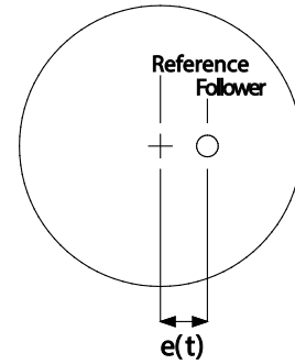
Figure 2: Compensatory display.
