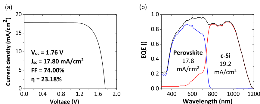
FIGURE 8 (a) Current density-voltage (JV) curve and (b) external quantum efficiency (EQE) curve of 2T perovskite/c-Si tandem solar cell with poly-SiO x passivated c-Si bottom cell. The corresponding device structure is shown in Figure 1. The blue, red, and black curves represent EQE spectra of perovskite top cell, c-Si bottom cell, and tandem cell, respectively. The area covered by the blue line indicates the photo-current density generated by the perovskite top cell, whereas the area covered by the red line indicates the photo-current density generated by c-Si bottom cell. [Colour figure can be viewed at wileyonlinelibrary.com ]
