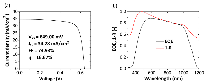
FIGURE 7 (a) Current density–voltage characteristic and (b) external quantum efficiency (EQE) and 1-Reflectance (1-R) spectra of the single junction c-Si solar cell with front side flat n-type poly-SiO x and rear side textured p-type poly-SiO x . The schematic of the corresponding structure is given in Figure 1. [Colour figure can be viewed at wileyonlinelibrary.com ]
