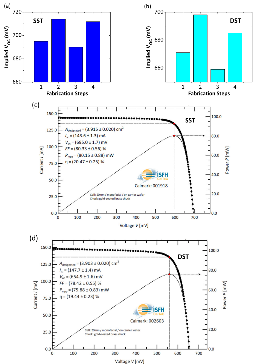
FIGURE 5 (a–b) The evolution in passivation quality ( iV_{oc} ) after specific steps of single-side textured (SST) and double-side textured (DST) solar cell fabrication: (1) annealing, (2) hydrogenation, (3) Transparent conductive oxide (TCO) deposition, and (4) hydrogen annealing; (c–d) certified current–voltage and power–voltage curves of the best SST and DST poly-SiO x passivated c-Si solar cell. Sketches of SST and DST solar cells are reported in Figure 2. [Colour figure can be viewed at wileyonlinelibrary.com ]
