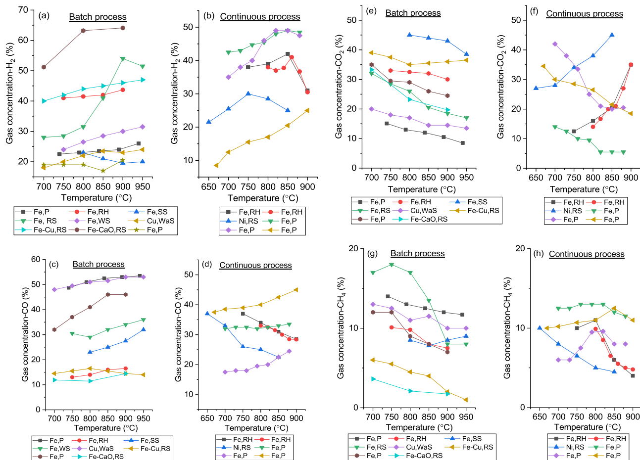
Fig. 4. Effect of temperature on (a/b) \text{H}_2 , (c/d) \text{CO} , (e/f) \text{CO}_2 and (g/h) \text{CH}_4 concentration (%) for different OCs and feedstock using batch/continuous processes, respectively [29,32,39,67,68,73,74,77–79,81–83].
