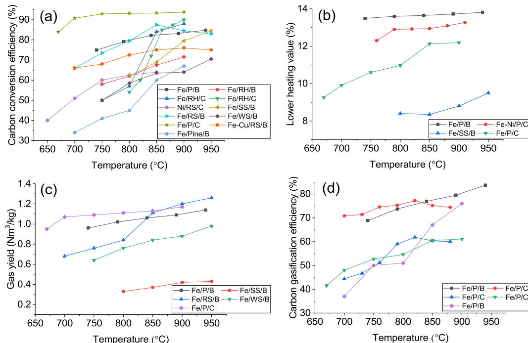
Fig. 5. Effect of temperature on CCE/LHV/CGE/gas yield for different OCs and feedstocks [29,32,39,67,68,73,74,77–79,81–83].
