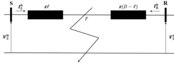
b): Equivalent negative sequence circuit of the faulted line.
