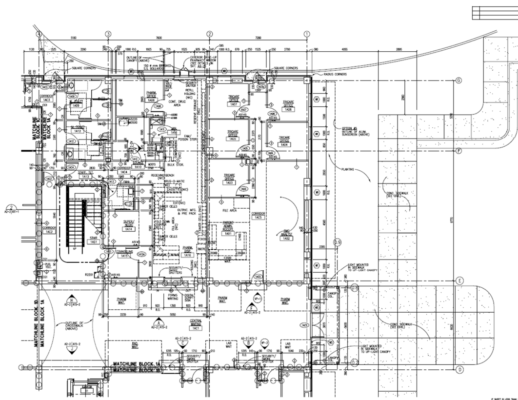
Figure 15. Typical floor view of the clinic building.
