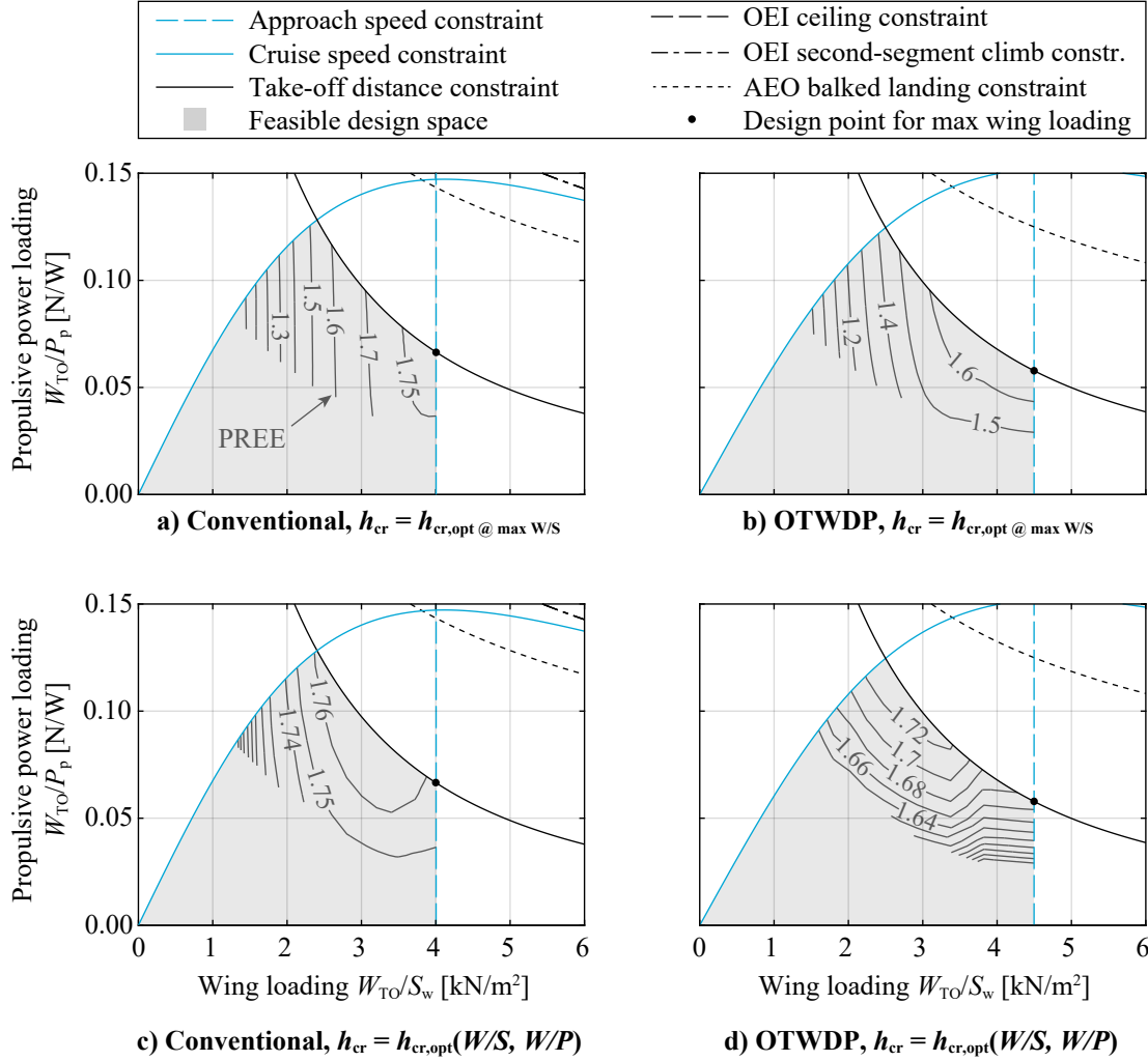
Fig. 7 Propulsive power-loading constraint diagrams of the conventional reference aircraft (left) and the hybrid-electric OTWDP variant (right), including contours of PREE obtained in the feasible design space for a fixed (top) and optimized (bottom) cruise altitude ( M_{cr} = 0.41 ).
