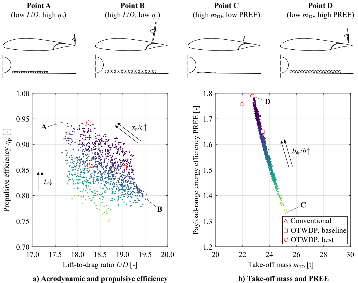
Fig. 12 Top-level aircraft performance metrics for various combinations of OTWDP geometrical design-parameter values, as obtained from the DoE. Darker colors indicate higher PREE values. Top sketches indicate the size and position of the OTWDP array, for four specific data points. M_{cr} = 0.41 , R = 825 nmi.
