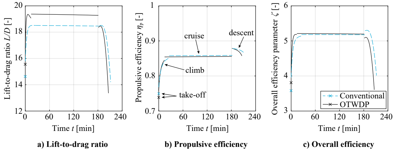
Fig. 9 Aerodynamic, propulsive, and overall efficiencies throughout the nominal mission ( M_{cr} = 0.41 , R = 825 nmi). Take-off values correspond to V_2 (i.e., after liftoff). Diversion and loiter not shown.
