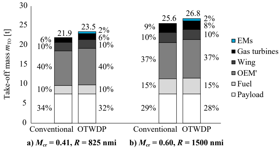
Fig. 10 Mass breakdown of the conventional and OTWDP configurations, for the short and long-range missions. Values are expressed in metric tons and as a percentage of take-off mass.
