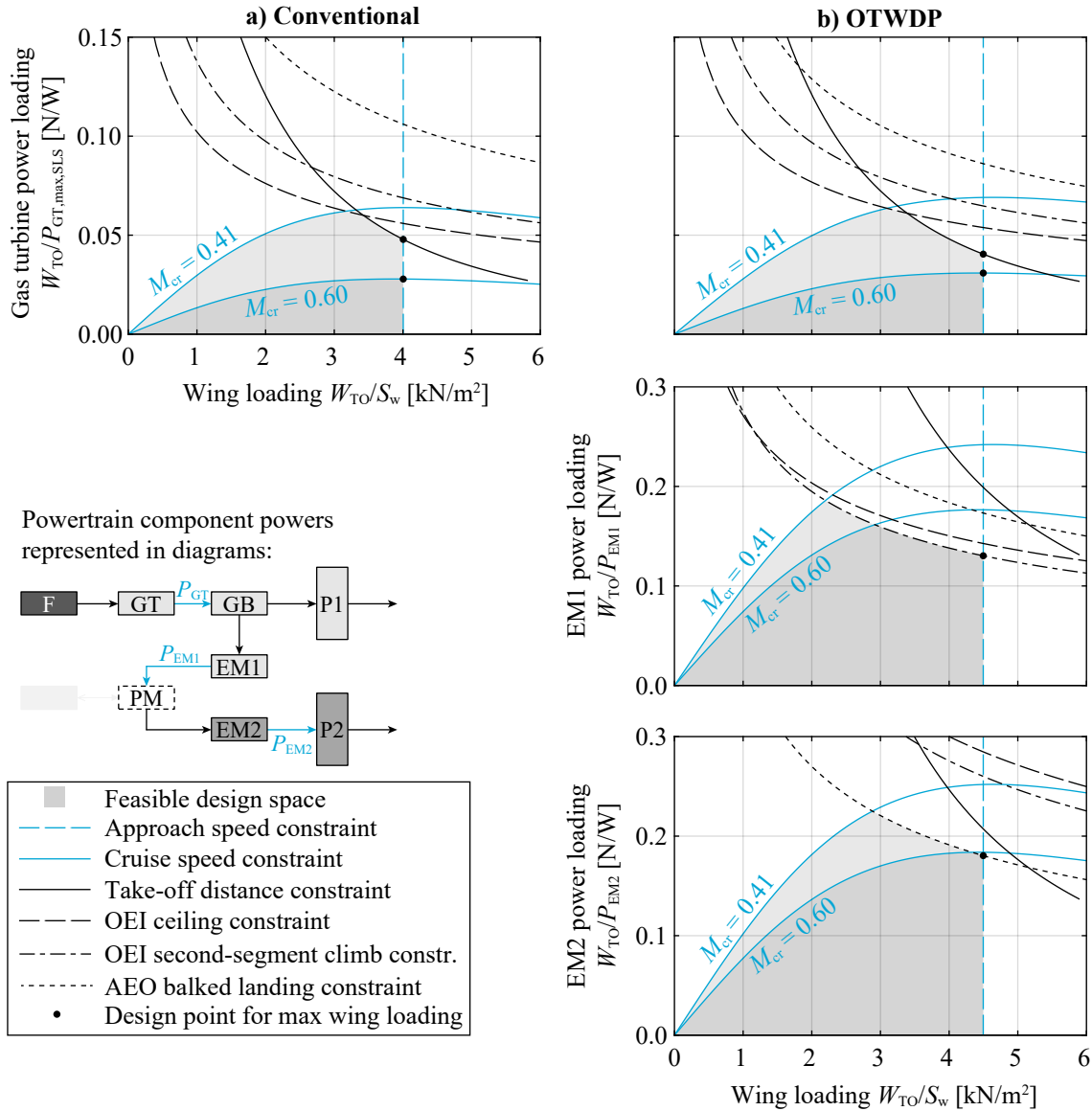
Fig. 8 Component power-loading constraint diagrams of the conventional reference aircraft (top left) and the hybrid-electric OTWDP variant (right).
