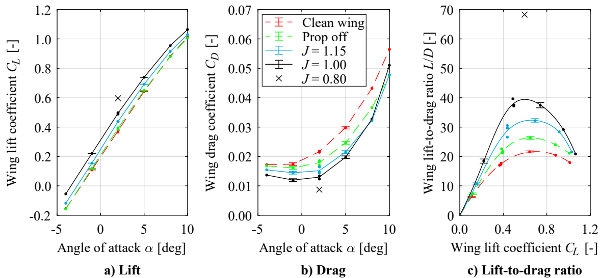
Fig. 4 Wing lift, drag, and lift-to-drag ratio polars. Data obtained from external balance measurements ( x_P/c = 0.8 , D_P/c = 0.68 ).
