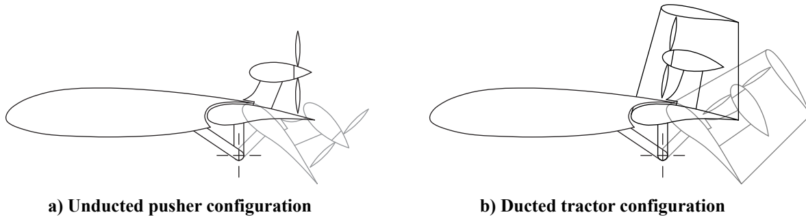
Fig. 6 Conceptual sketch of two OTWDP variants, including the position of the propeller in case of a \delta_f = 45^\circ flap deflection.
