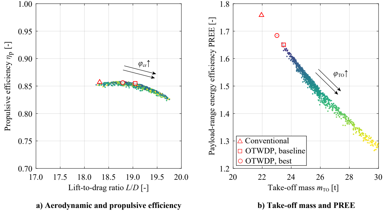
Fig. 13 Top-level aircraft performance metrics for various combinations of shaft power ratio \phi , as obtained from the DoE. Darker colors indicate higher PREE values. M_{cr} = 0.41 , R = 825 nmi.
