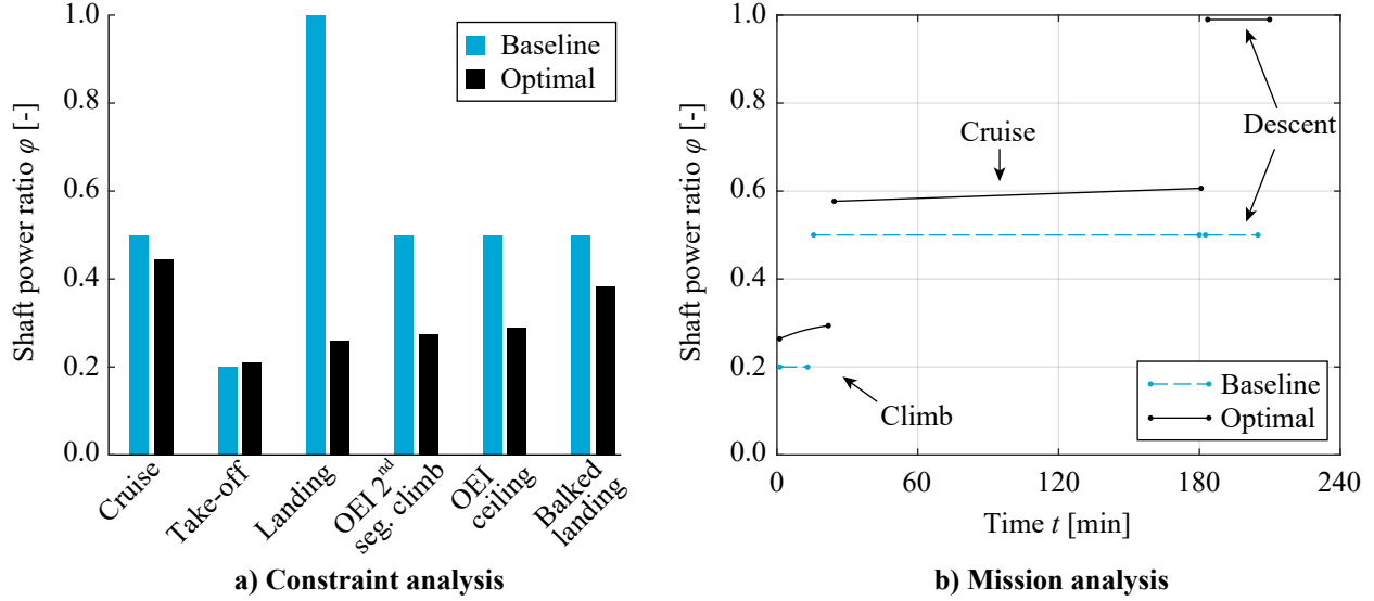
Fig. 14 Comparison of shaft-power-ratio values obtained for the OTWDP configuration in the performance constraints (left) and throughout the nominal mission (right). M_{cr} = 0.41 , R = 825 nmi.
