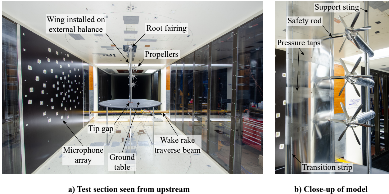
Fig. 2 Overview of the test section and wind-tunnel model used in the experimental campaign.
