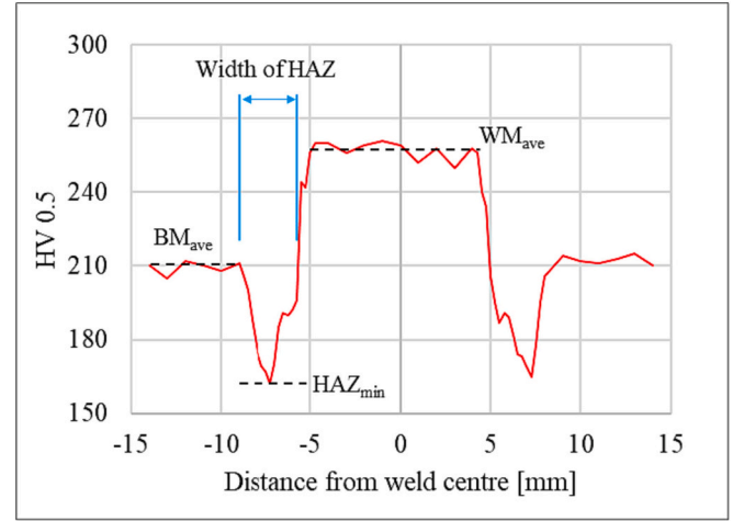
Fig. 9. Evaluation of the hardness result.
