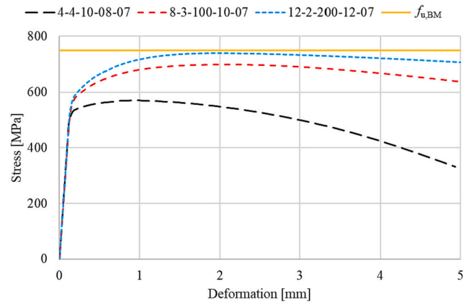
Fig. 5. Stress-deformation relationship.
