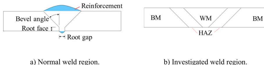
Fig. 1. Weld details.
