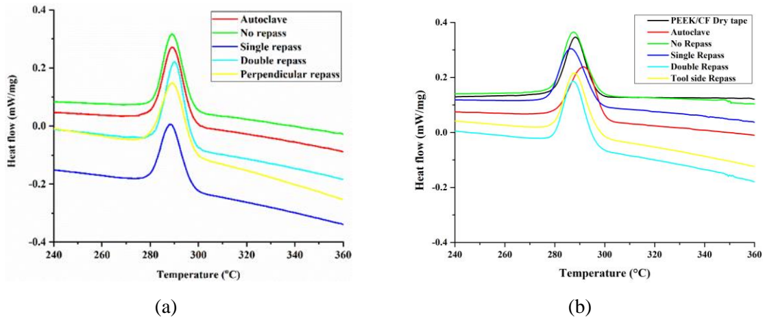
Fig. 7. Heat flow (exo \uparrow ) to temperature curves (Thermal transitions): (a) Thermal transitions for UD [0^\circ]_{16} laminates and (b) Thermal transitions for angle ply [\pm 45^\circ]_{4s} laminates.
