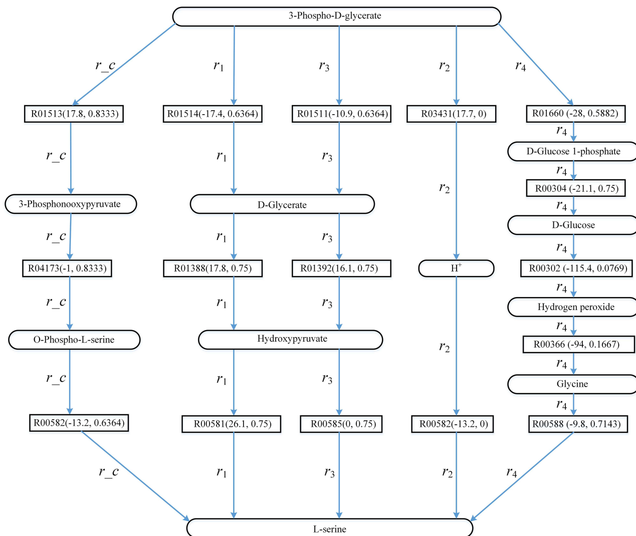
Fig 4. Computed pathways for L-serine biosynthesis: r_1 , r_2 , r_3 and r_4 . Rectangles represent reaction edges, and the data in parentheses denote the value \Delta G'_r of reaction and the compound similarity respectively.
