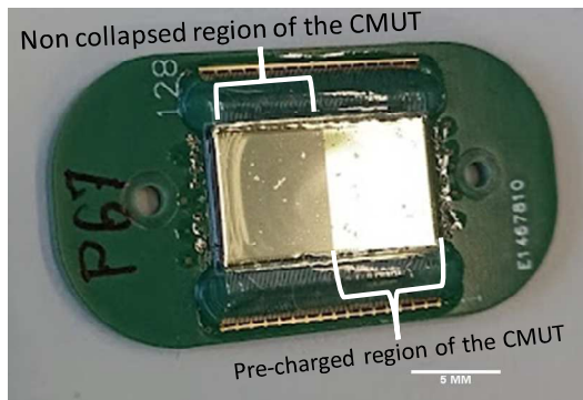
Fig 2. Pre-charged CMUT array after charging. The device in collapse-mode can be seen clearly in the ambient light reflection,
