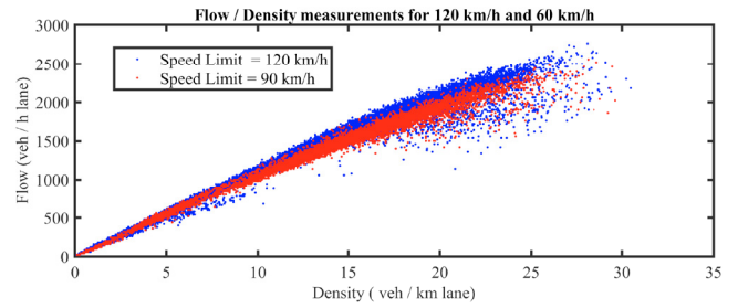
Fig. 4. Traffic data for Link 15 with V_{c,i}(k) = 120 km/h (blue) and V_{c,i}(k) = 90 km/h (red).
