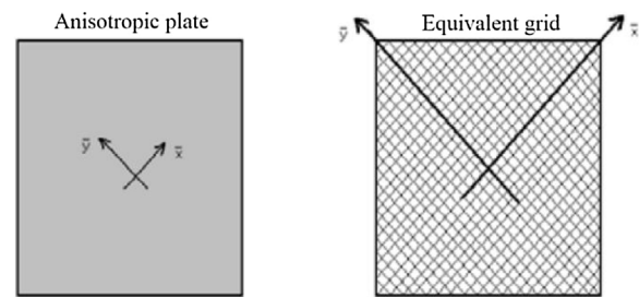
Fig. 10. Analogy between plates and grids.
