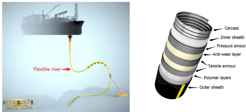
Fig. 1. Flexible riser and its layer configuration.
