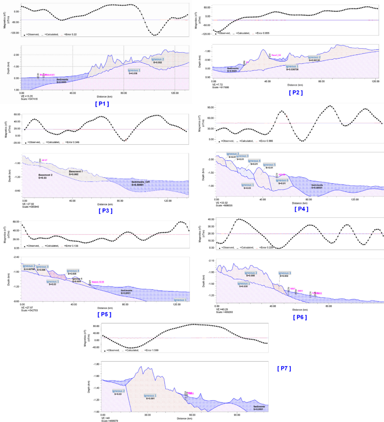
FIGURE 11 | The 2D inverted magnetic models.
