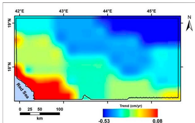
FIGURE 5 | Color-coded \Delta TWS trend during the period 04/2002–12/2021 from averaging of the CSR-M data.
