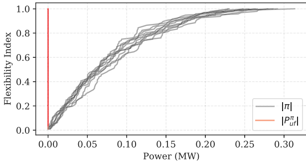
Fig. 15. The ECDF for the signals in Fig. 14 shows the flexibility index is 1, implying a totally flexible system.
