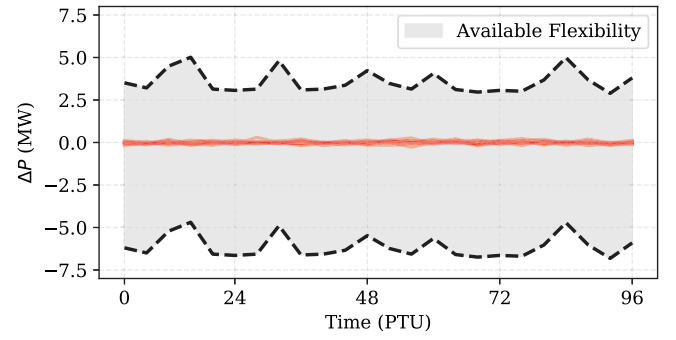
Fig. 5. Assessing flexibility using Minkowski Summation. The red lines indicate the FR signal scenario set. The black dashed lines indicate the upper and lower levels of allowable power excursion calculated using the Minkowski method. The available flexibility bound is calculated in each PTU for the next PTU.
