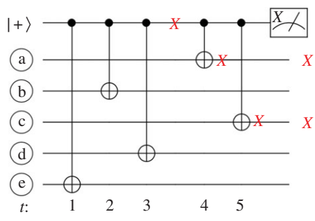
Figure 8. Circuit for measuring a weight-5 X -check. A single X fault occurring after the third CNOT gate can propagate to two data qubits resulting in two outgoing X errors. (Online version in colour.)
