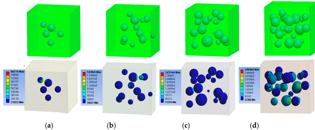
Figure 11. Volume element models and transient mechanical simulation results of phosphor/silicone composites (a) 5%; (b) 10%; (c) 15%; (d) 20%.
