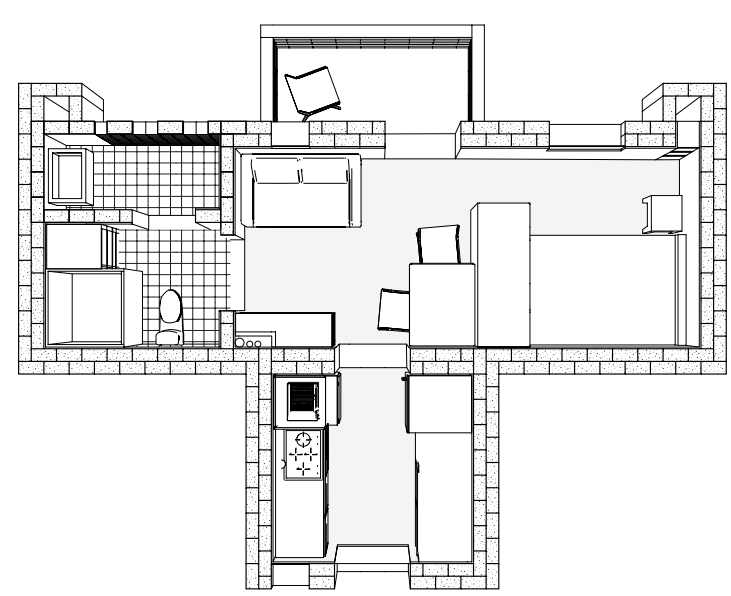
Apartment 1 26 m2 1:100
