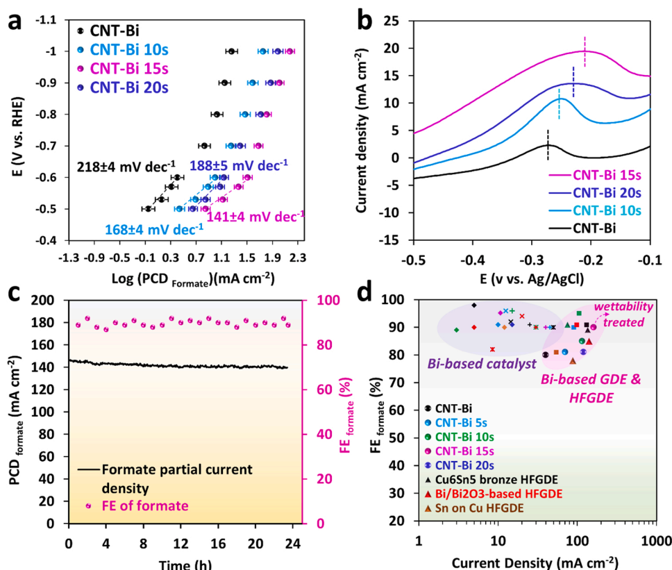
Fig. 4. a) Tafel plots of formate for dual-layer HFGDEs; b) Single oxidative LSV scans at 50 mV s -1 in N 2 -saturated 0.1 M; c) 24 h stability test at -1.0 V vs. RHE: faradaic efficiency and formate partial current density in the flow reactor with CNT-Bi 15 s dual-layer HFGDE; d) CO 2 RR performance comparison of dual-layer HFGDEs with other Bi-based catalysts and GDEs/HFGDEs for formate production in neutral (bicarbonate) electrolytes with the same concentration (more details on CO 2 RR performance and electrolyte type in Table S2).
