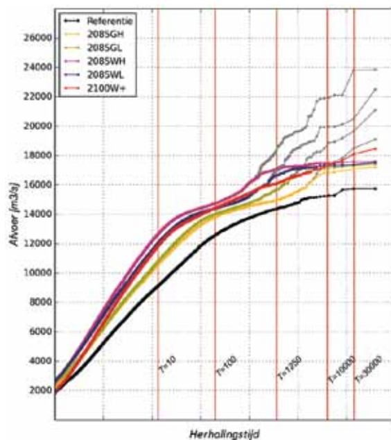
Figure 1 Development of the relationship between exceedance probability (expressed as average recurrence time) and the discharge of the Rhine at Lobith in 2085 as potentially produced in the catchment (in gray) and the actually expected discharge at Lobith taking if flooding in Germany is taken into account (in colour) for the four KNMI'14 scenarios and the KNMI'06 W+ scenario (Klijn et al. , 2015).
