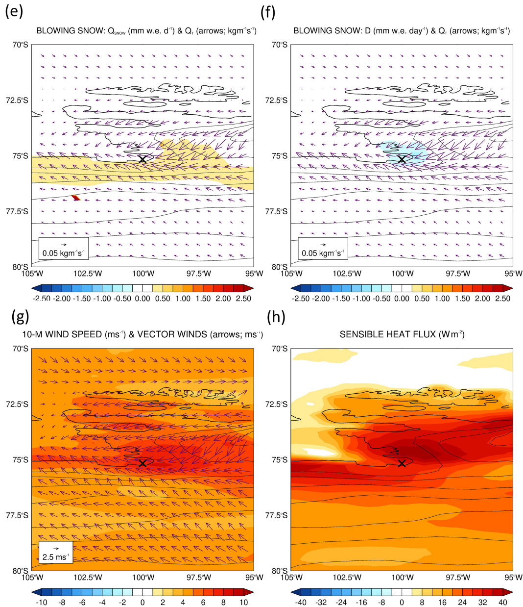
Figure 4. Composite difference between Foehn and no-Foehn timestamps for 1980–2020. (a) Storage or accumulation rate of snow at the surface ( S in Eq. (2); mm w.e. \text{d}^{-1} ), (b) precipitation and snowfall rate ( P ; mm w.e. \text{d}^{-1} ), (c) surface sublimation rate ( Q_{\text{surf}} ; mm w.e. \text{d}^{-1} ; positive values indicate deposition to the surface, and negative values indicate sublimation), (d) snowmelt rate ( M ; mm w.e. \text{d}^{-1} ; positive values indicate melting), (e) blowing-snow sublimation rate ( Q_{\text{snow}} ; mm w.e. \text{d}^{-1} ; positive values indicate sublimation), (f) blowing-snow divergence rate ( D ; mm w.e. \text{d}^{-1} ), (g) 10 m wind speed (shading; \text{m s}^{-1} ) and (h) instantaneous surface sensible heat flux ( \text{W m}^{-2} , positive if downwards towards the surface). The arrows in (e) and (g) give the 10 m horizontal wind vectors ( \text{m s}^{-1} ), while in (e) and (f) they show the blowing-snow transport rate ( Q_t ; \text{kg m}^{-1} \text{s}^{-1} ).
