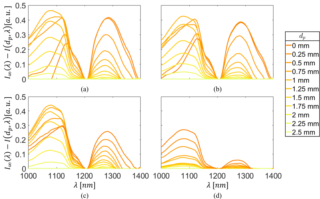
Figure 5: Normalized reflectance spectra ( \lambda_0 = 1211 nm) for different distances to the interface relative to the normalized reflectance spectrum of the pure cancellous bone-mimicking phantom with (a) diffuse light emission and forward light collection, perpendicular breach (b) forward light emission and forward light collection (conventional parallel DRS), perpendicular breach (c) diffuse light emission and sideways light collection, parallel breach (d) diffuse light emission and forward light collection, parallel breach.
