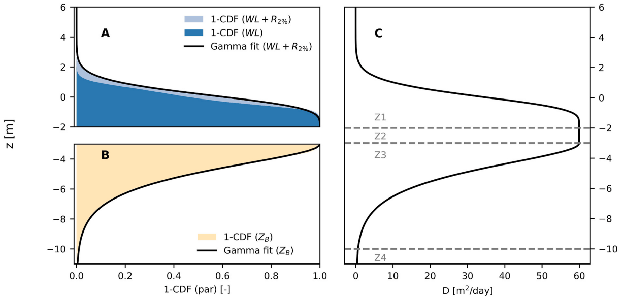
Fig. 2. A) Example survival functions of WL (water level and surge) and WL + R_{2\%} (water level, surge, and wave runup). B) Example survival function of Z_B whereby breaker index \gamma is set to 0.44 (Miche, 1954). C) Resulting diffusion coefficient D(z') with D_{MAX} = 60 m^2/day as adopted from de Vriend et al. (1993). Z_1 , Z_2 , Z_3 and Z_4 indicate zones as referred to in the main text, divided by the grey dashed lines. The CDFs and zonation in this example are based on the hydrodynamic data of 1985–2018 at the Dutch IJmuiden measuring station.
